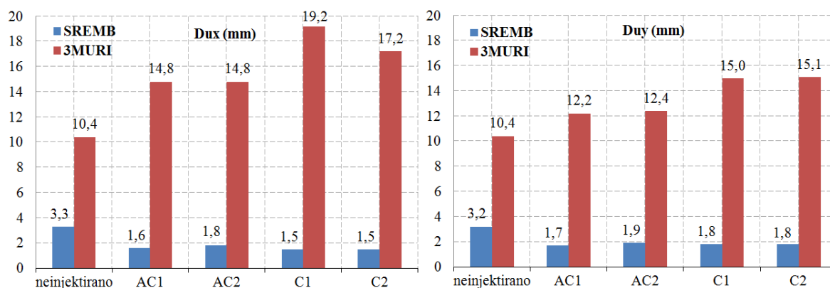
Slika 6.41: Kapaciteta konstrukcije v smislu pomika D_u pri MSN pri izračunu s SREMB in 3MURI za smer X in Y Fig. 6.41: Capacity of a structure in terms of displacement D_u at ULS calculated by SREMB and 3MURI in X and Y direction
