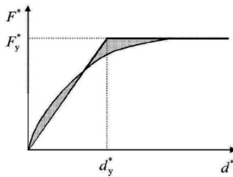
Slika 6.13: Dejanski in idealiziran diagram sila-pomik sistema SDOF Fig. 6.13: Actual and idealized diagram force-displacement of a SDOF system
