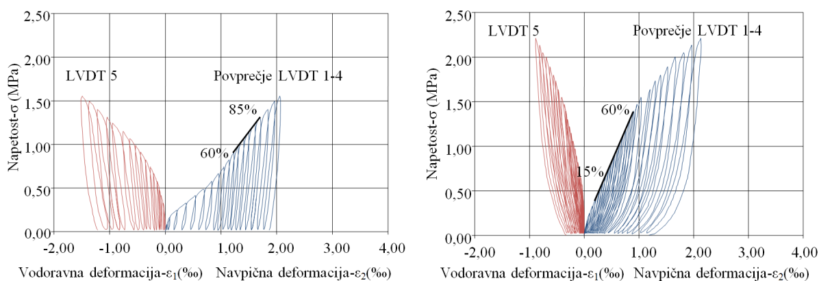
Slika 5.21: Rezultati preiskave zidu 5-C2 z jeklenimi blazinami pred (levo) in po injektiranju (desno) Fig. 5.21: Results of the double flat-jack test of the wall 5-C2 before (left) and after grout injection (right)
