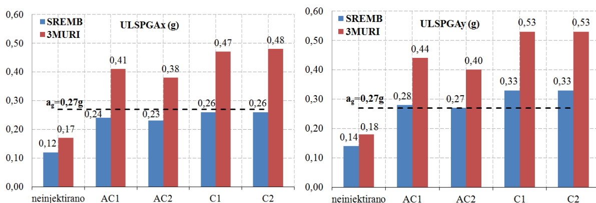
Slika 6.42: Mejni pospeški tal ULSPGA, izračunani s SREMB in 3MURI za smer X in Y Fig. 6.42: Limit ground acceleration ULSPGA calculated by SREMB and 3MURI in X and Y direction
