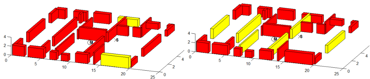
Slika 6.26: Mehanizem porušitve v X (levo) in Y smeri (desno) za stanje po injektiranju z C1 Fig. 6.26: Failure mode in X (left) and Y direction (right) for the construction grouted by C1
