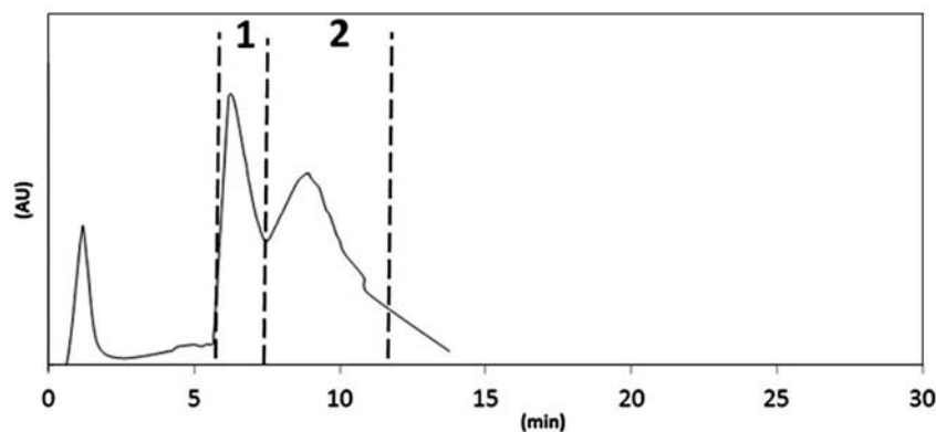
Fig. 13. Chromatogram obtained on pilot preparative to production scale SFC, 1 st fraction and 2 nd fraction; temperature of the column was 45 °C, column inlet pressure was 180 bar. Modifier was added after injection at mass fraction of approximately 6%, mobile phase flow was approx. 1.2 kg/h (measured on the flow meter),
