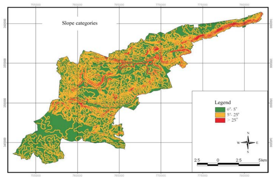
Fig.6: Slope categories in Aggtelek National Park.
