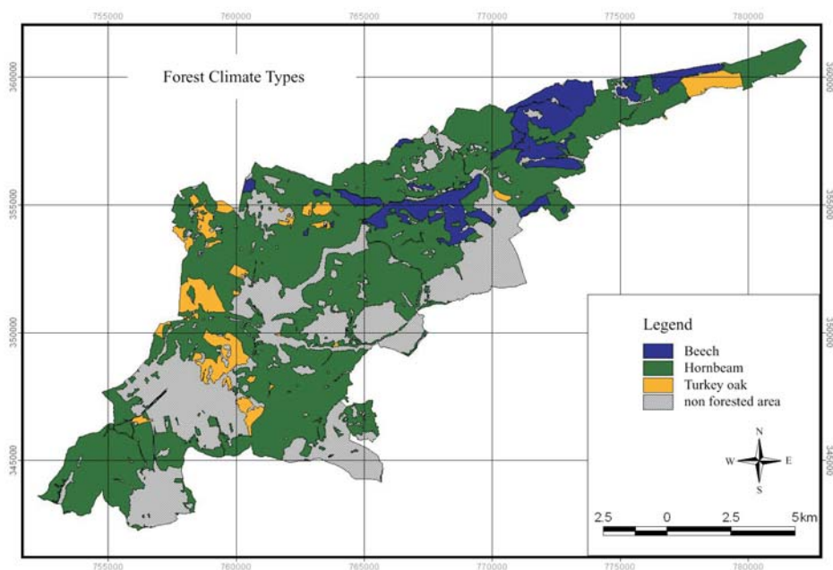
Fig. 2: Forest climate types in Aggtelek National Park .
