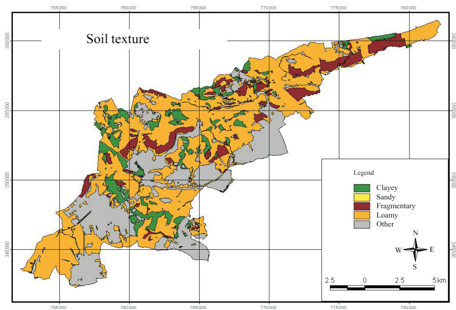
Fig. 8: Soil texture in Aggtelek National Park.
