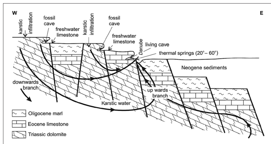
Fig. 2: Sketch of the Buda Thermal Spring system illustrating the mixing of ascending and descending waters (Leél-Össy & Surányi 2003).
