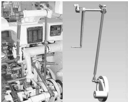
Fig. 5. Ejection system
