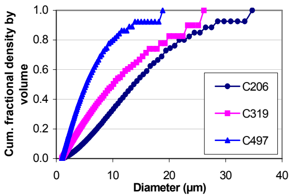
Fig. 1. Cumulative particle size distribution (PSD) curves for simulated cements.
