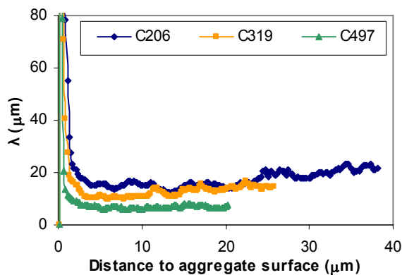
Fig. 12. Gradients in mean free spacing \lambda for different types of cement ( w/c = 0.2 ).
