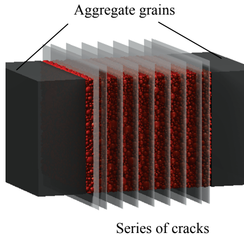
Fig. 13. Evaluation of cracks interfering with UCN to provide gradient information on local self-healing capacity.
