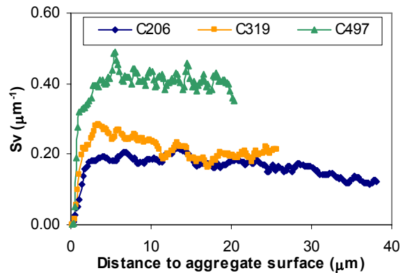
Fig. 10. Gradients in S_V of UCN for three cement finenesses (w/c = 0.2).
