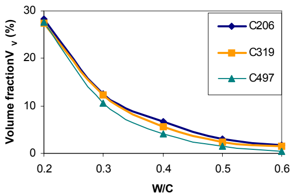
Fig. 3. Volume fraction of UCN for three cements with different w/c ratios.
