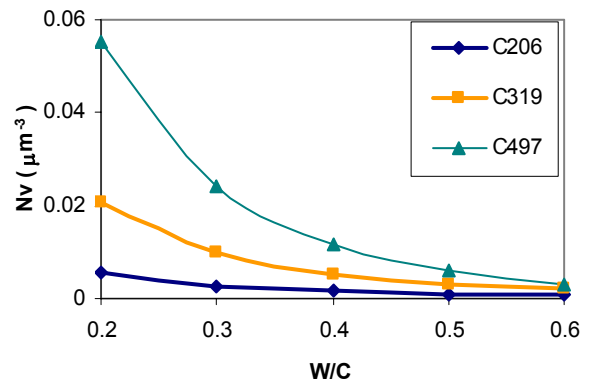
Fig. 4. Number of UCN per unit volume for three cements with different w/c ratios.
