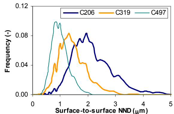
Fig. 5. Probability density functions of NNSSS of UCN in three cement pastes (w/c = 0.2).
