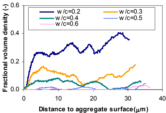
Fig. 7. Gradients in V_V of UCN in C497 for five w/c ratios.
