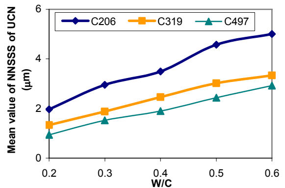
Fig. 6. Mean values of NNSSS-curves of three cements paste with increasing w/c ratios.
