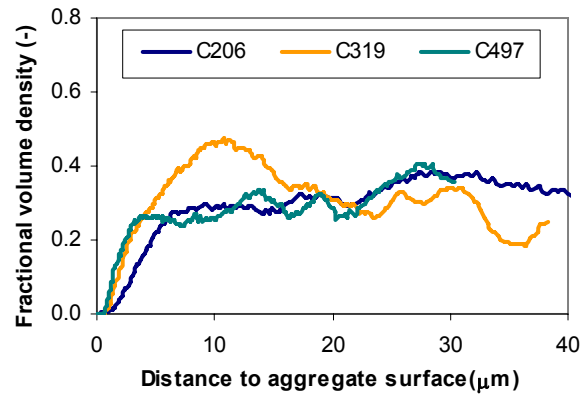
Fig. 8. Gradient in V_V of UCN for three cement paste finenesses (w/c = 0.2).
