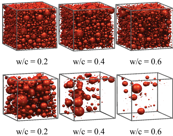
Fig. 2. Cement pastes (top) and UCN (bottom) of C206 after 1 year of hydration.
