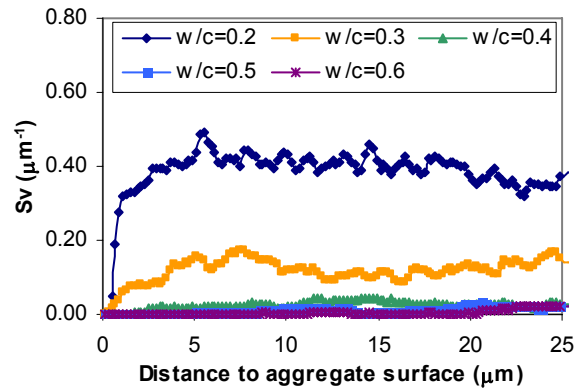
Fig. 9. Gradients in S_V of UCN of five w/c ratios (C497).
