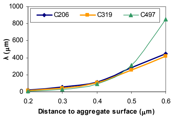
Fig. 11. Mean free spacing \lambda for different types of cement and different w/c -ratios.
