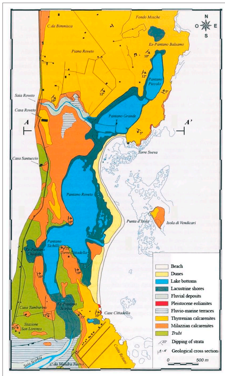
Fig. 2: Geological map of Venticari area.
