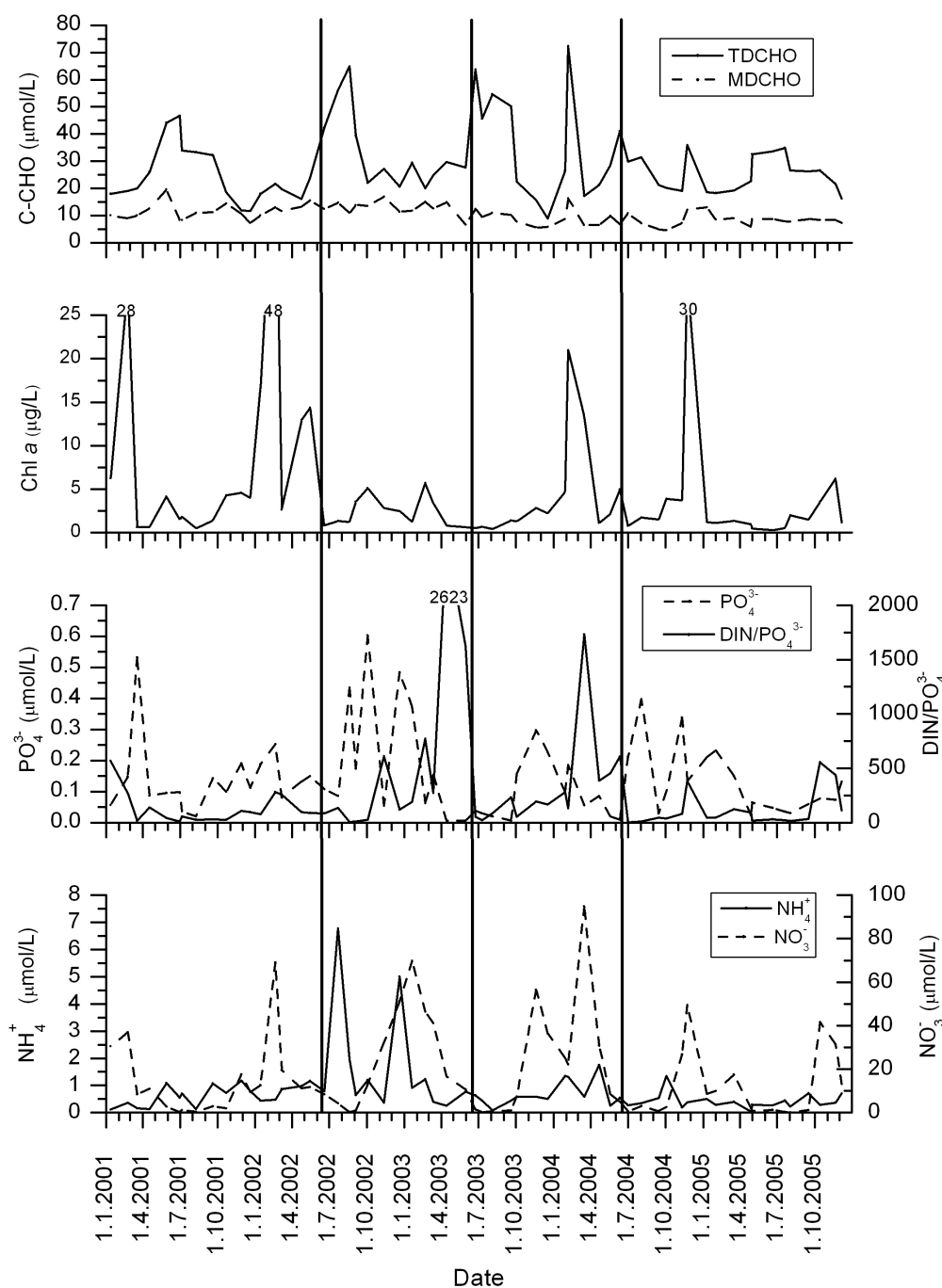
Figure 2. Variations of total dissolved carbohydrates (TDCHO), dissolved monosaccharides (MDCHO), chlorophyll a , nitrate, ammonium, phosphate and DIN/ \text{PO}_4^{3-} ratio in the surface layer (0.5 m) of northern Adriatic off Pesaro. Vertical lines indicate the occurrence of macroaggregates.
