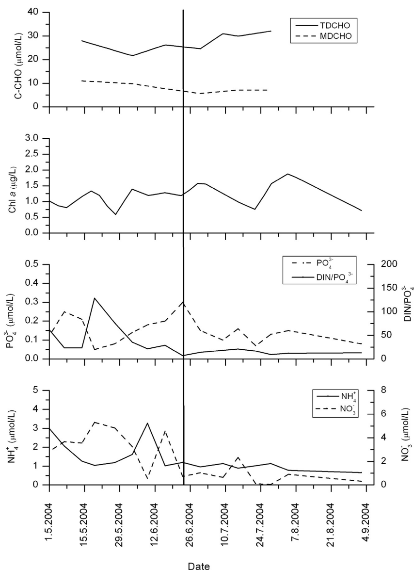
Figure 3. Variations of total dissolved carbohydrates (TDCHO), dissolved monosaccharides (MDCHO), chlorophyll a , nitrate, ammonium, dissolved inorganic nitrogen (DIN), phosphate and DIN/ \text{PO}_4^{3-} ratio in the surface layer (0.5 m) of the Gulf of Trieste. Vertical line indicates the occurrence of macroaggregates (from Kovac et al.). 16
