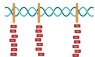
Targeted sequencing
