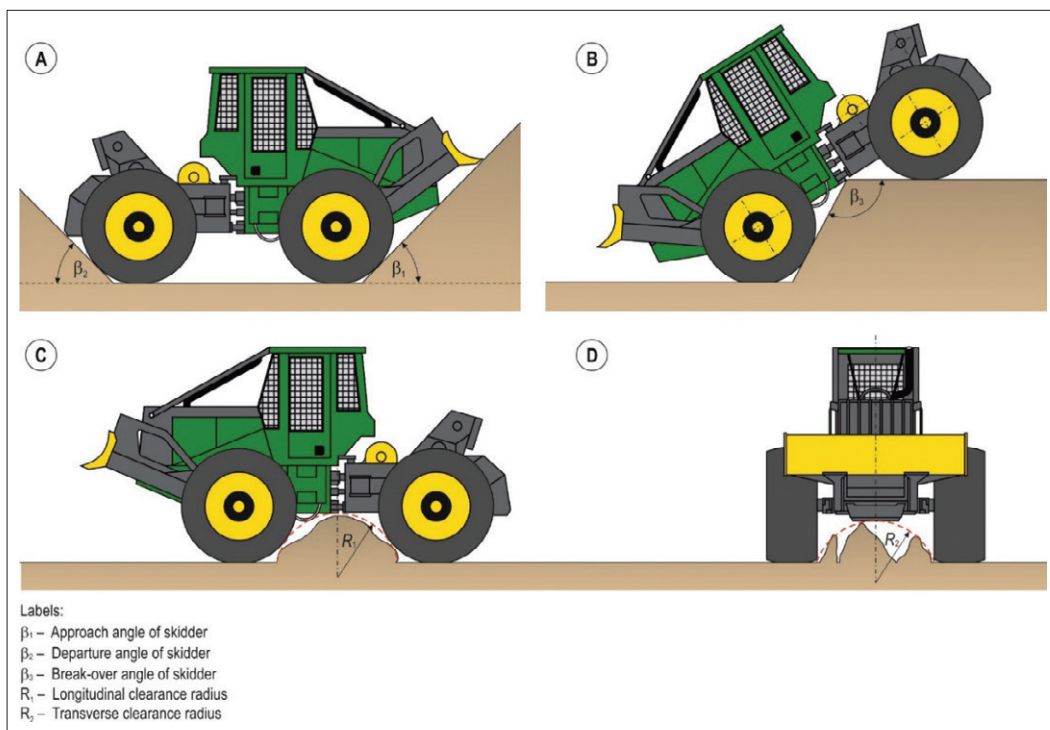
Slika 3: Vpliv kotov zmožnosti manevriranja in polmera manevrskega prostora na mobilnost vlačilca Figure 3: Impact of maneuverability angles and clearance radiuses on skidder mobility
