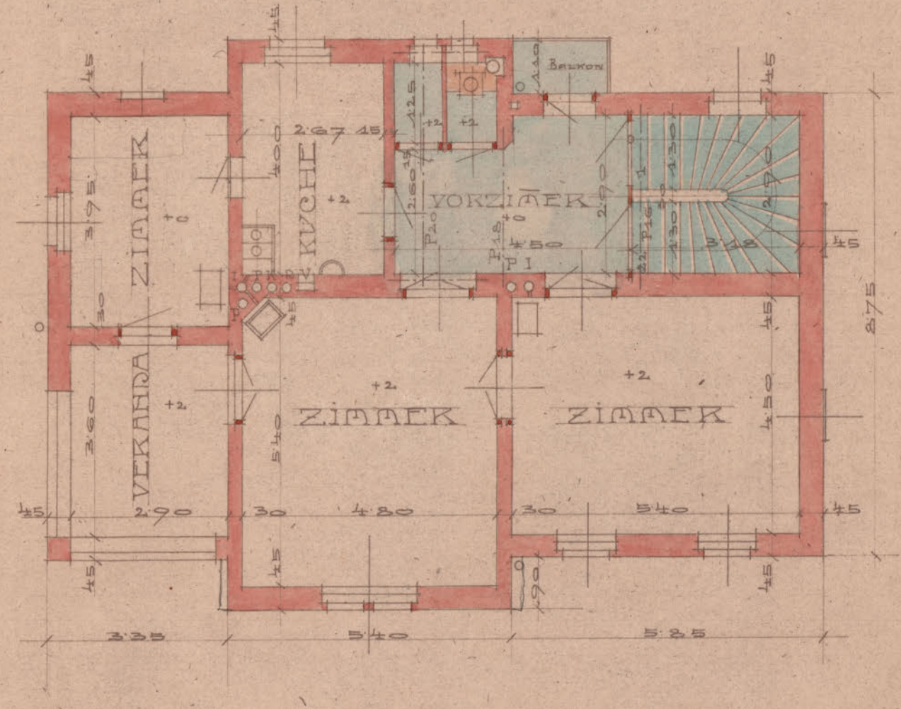
I. STOCK
