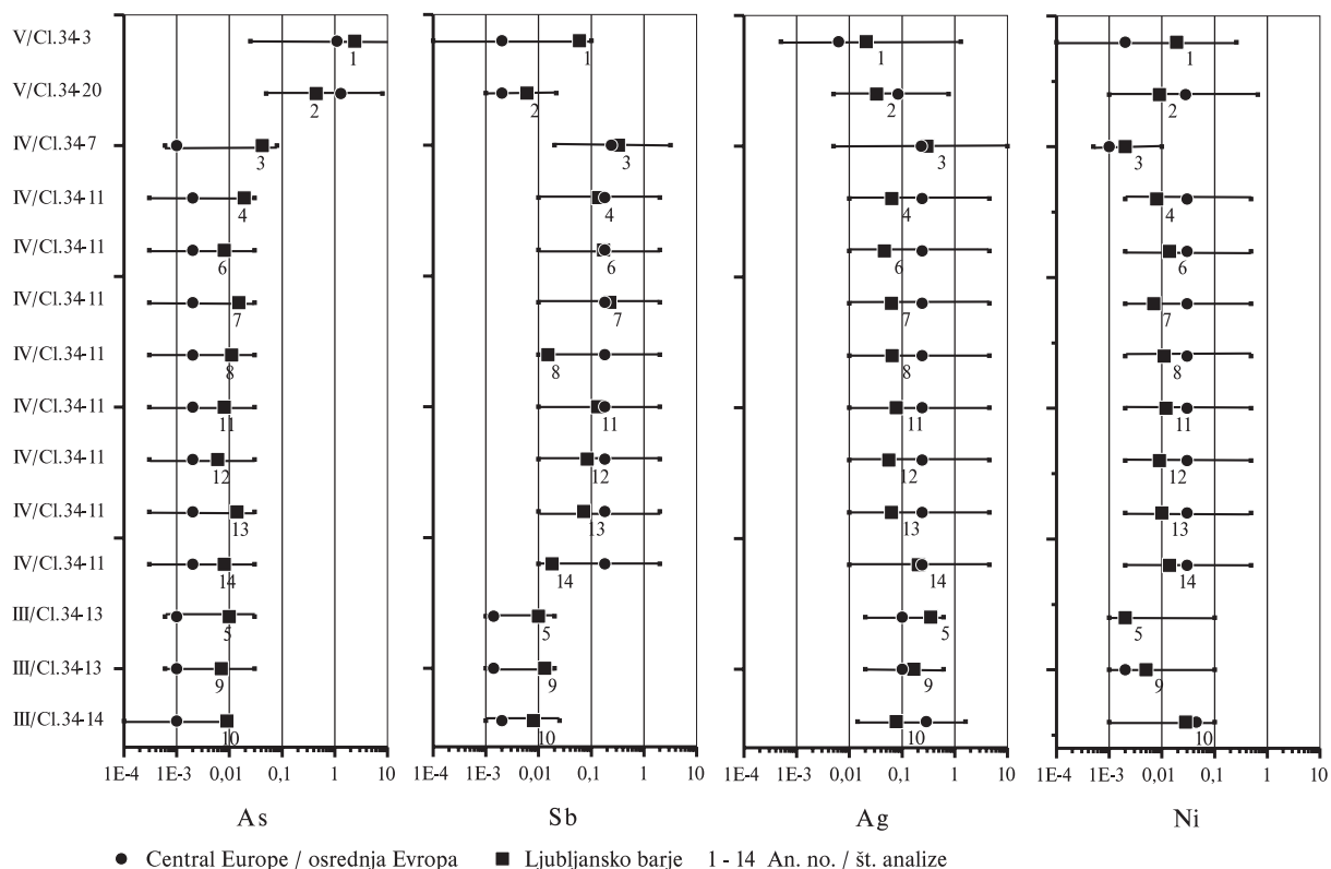
Fig. 3: Absolute values of arsenic, antimony, silver and nickel in 14 copper artefacts from the Ljubljansko barje compared with average values in artefacts from Central Europe and classification of Ljubljana artefacts to various copper types (according to Krause 2003, 91, Fig. 41).
