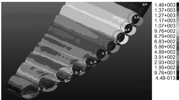
Fig. 18. Horizontal ribs model FEM analysis with damping and fabric element: displacements in mm
