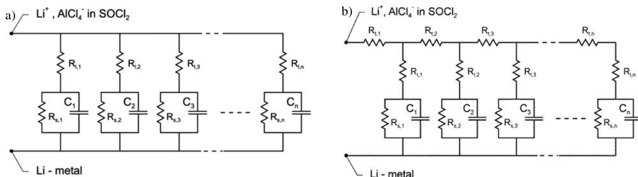
Figure 9. Electrical circuits tested as models of the LiCl layer. Fig. 9a is simulating the »simple crack« model of Fig. 8a, and 9b is another »ladder« type of circuit, which may respond as a CPA over certain frequency ranges dependent on the actual values of resistances and capacitances. Even higher degrees of branching are necessary in order to simulate the observed CPE behaviour pointing to a much branched crack and tunnel system.
