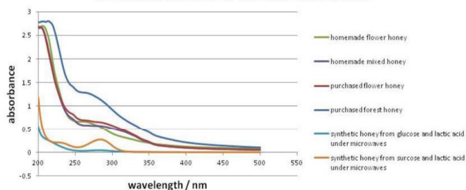
COMPARISON OF SPECTRA OF DIFFERENT HONEY SAMPLES
