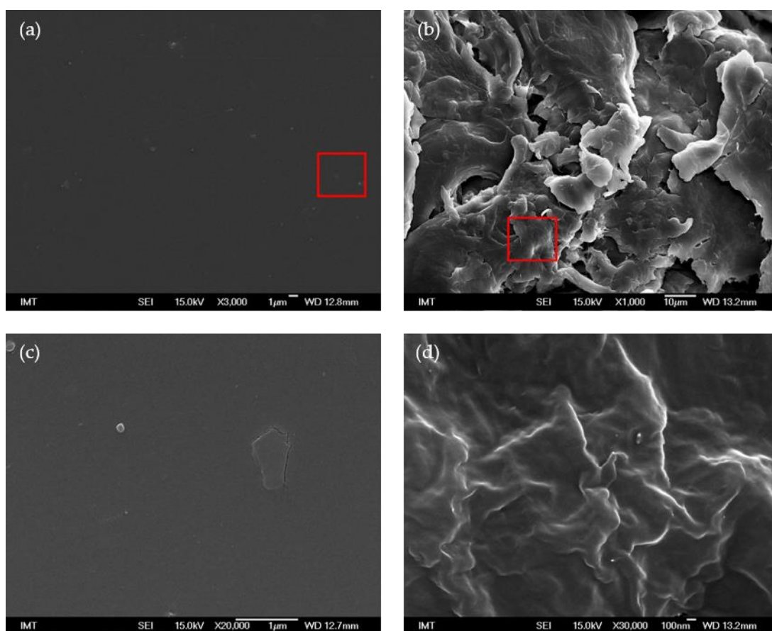
Figure 1: Pre-cut fragment (5 mm - 1 mm) and cryomilled particle (1 mm - 100 \mu\text{m} ) of PET under SEM microscope at 3 000 x magnification (a), 1 000 x magnification (b), 20 000 x magnification (c) and 30 000 x magnification (d). Red rectangles in (a) and (b) indicate the areas containing the structures shown in (c) and (d).
