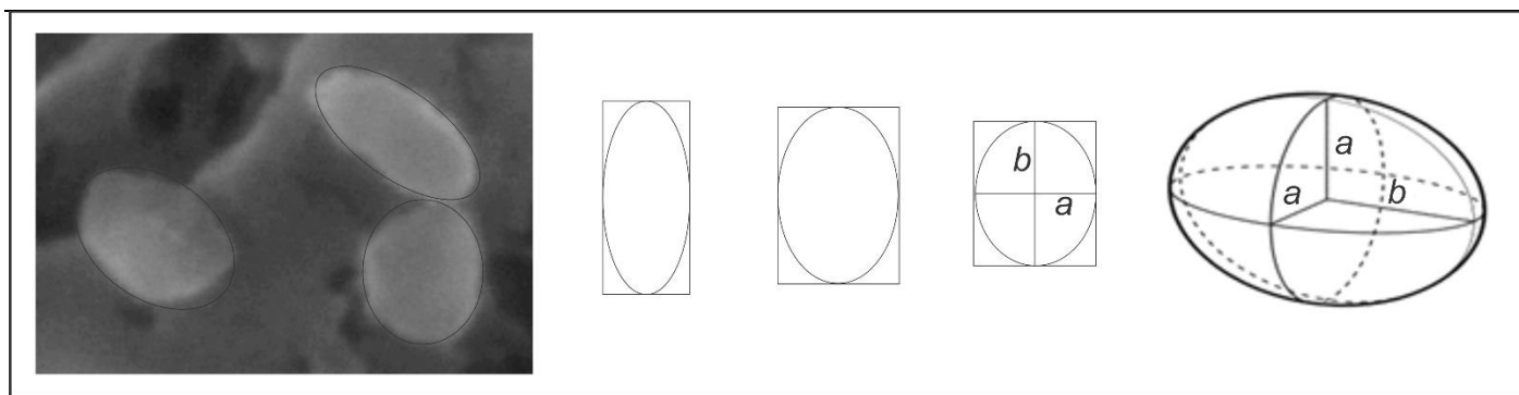
Figure 2. Fitting of the EV contours with prolate spheroid and determination of the semiaxes marked a and b .
