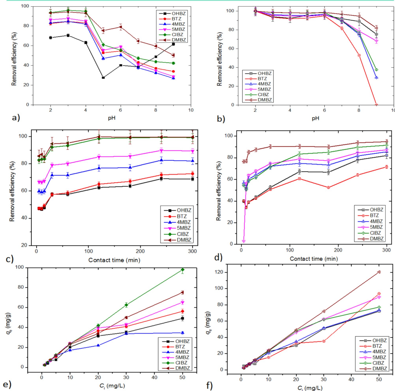
Figure 1: Influence of the pH value on removal efficiency on (a) WpOH; (b) AsPhA Influence of contact time on removal efficiency on (c) WpOH and (d) AsPhA Influence of initial concentration on adsorption capacity on (e) WpOH and (f) AsPhA
