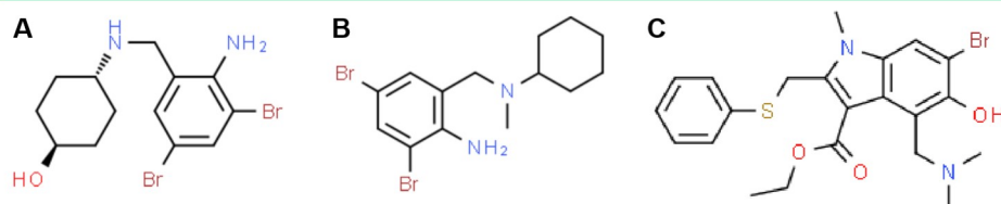
Figure 1: Ambroxol (a); Bromhexine (b); Umifenovir (c)
