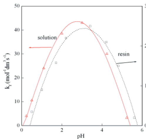
Figure 6. pH profile of reaction between IACA and Pd(II) in solution and on resin; c_i = c_{Pd} = 1 \times 10^{-5} M.
