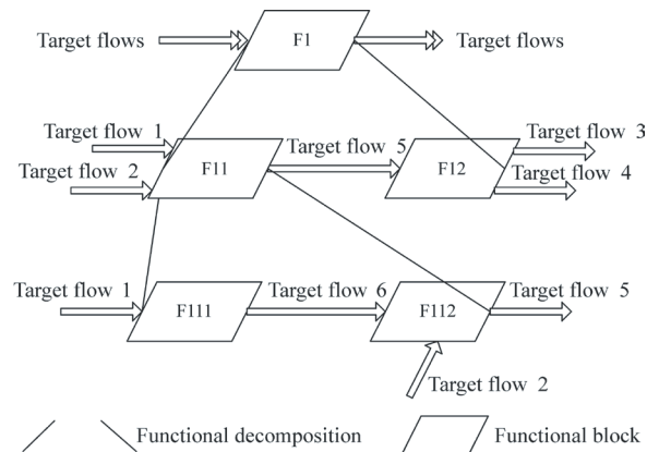
Fig. 3. Functional decomposition by tracing the change in target flows
