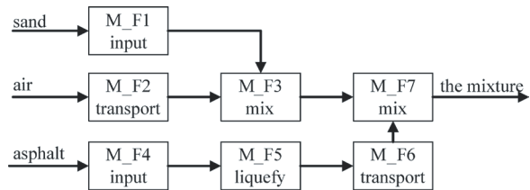
Fig. 12. Function-structure of the M_subsystem
