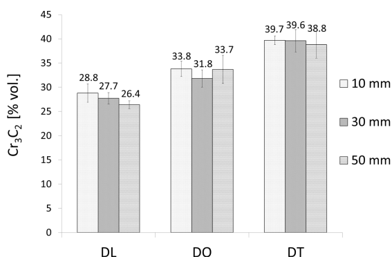
Fig. 11. Cr_3C_2 particles embedded in the Cr_3C_2-25(Ni20Cr) coatings (% vol.)
