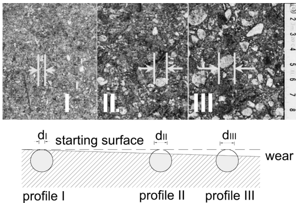
Fig. 2. The level of wear of the existing base concrete in the control profiles, in a distance from the chute of: (I) 1 m; (II) 7 m; (III) 13 m
