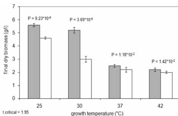
Figure 1: Final dry bacterial biomass production at different growth temperatures. At immediate induction (grey bars) more biomass per litre was produced than at delayed induction (white bars). Statistical analysis (T-test; P value) of 15 independent replicas showed that at all temperatures, the differences between the immediate and late induction regime regarding final biomass were significant.
