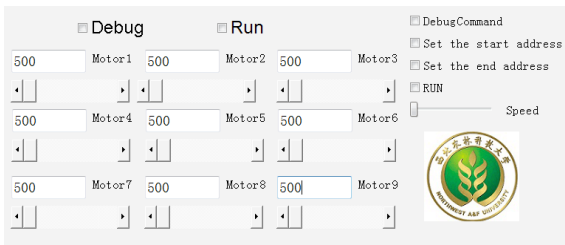
Fig. 19. Software interface
