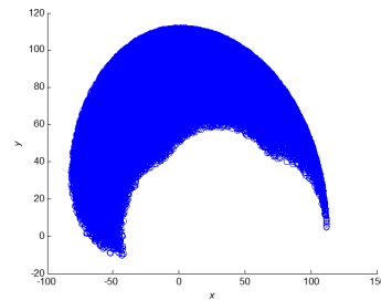
Fig. 13. Fingertip workspace
