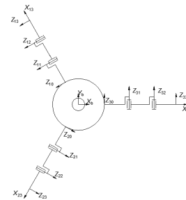
Fig. 14. Whole-hand D-H coordinate system
