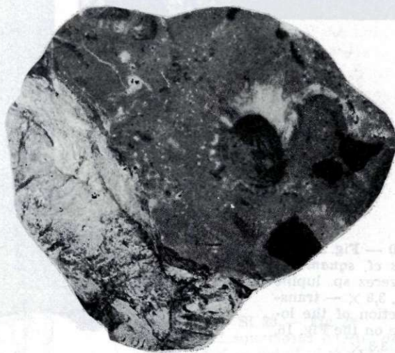
Sl. 17 — Fig. 17 Radiolites cf. squamosus d'Orb., prečni prerez spodnje lupine, senon, Nanos — transversal section through the lo- wer valve, Senonian, Nanos
