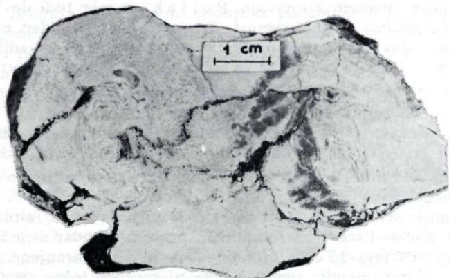
Sl. 32 — Fig. 32 Durania adriatica Polšak (levo — left), Durania sp. (desno — right), prereza spodnjih lupin, senon, Bilje — transversal section through the lower valves, Senonian, Bilje
