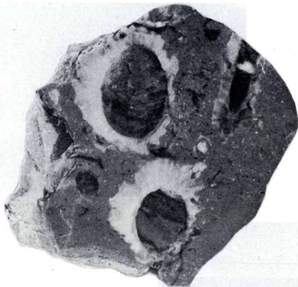
Sl. 16 — Fig. 16 Radiolites cf. squamosus d'Orb., dva prečna pre- reza spodnje lupine, se- non, Nanos — two trans- versal sections through the lower valve, Seno- nian, Nanos
