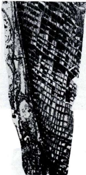
Sl. 41 — Fig. 41 Durania sp., radialni prerez spodnje lupine, 3,2 × — longitudinal section through the lower valve, 3,2 ×
