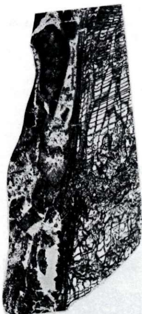
Sl. 36 — Fig. 36 Durania adriatica Polšak, radialni prerez lupine, 3,2 × — longitudinal section of the lower valve, 3.2 ×
