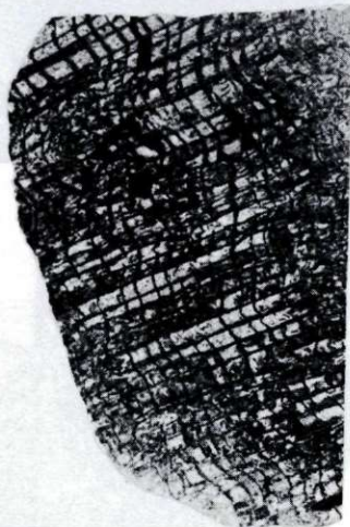
Sl. 42 — Fig. 42 Durania sp., tangencialni prerez spodnje lupine, senon, Bilje, 3,2 × — tangential section through the lower valve, Senonian, Bilje, 3,2 ×
