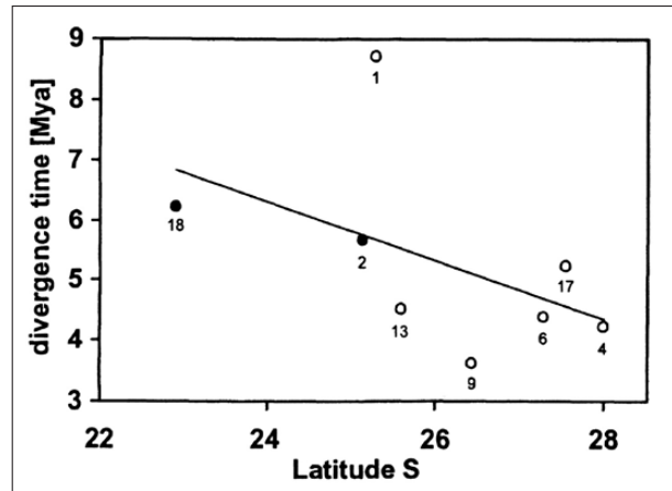
Fig. 1: Latitudinal variation in divergence times of eight sympatric sister pairs of stygobiotic dytiscid beetles in Western Australia. The open circles show species pairs belonging to the Bidessini; the black circles show species pairs belonging to the Hydroporini. Numbers refer to different calcrete aquifers (see Leys et al. 2003).
