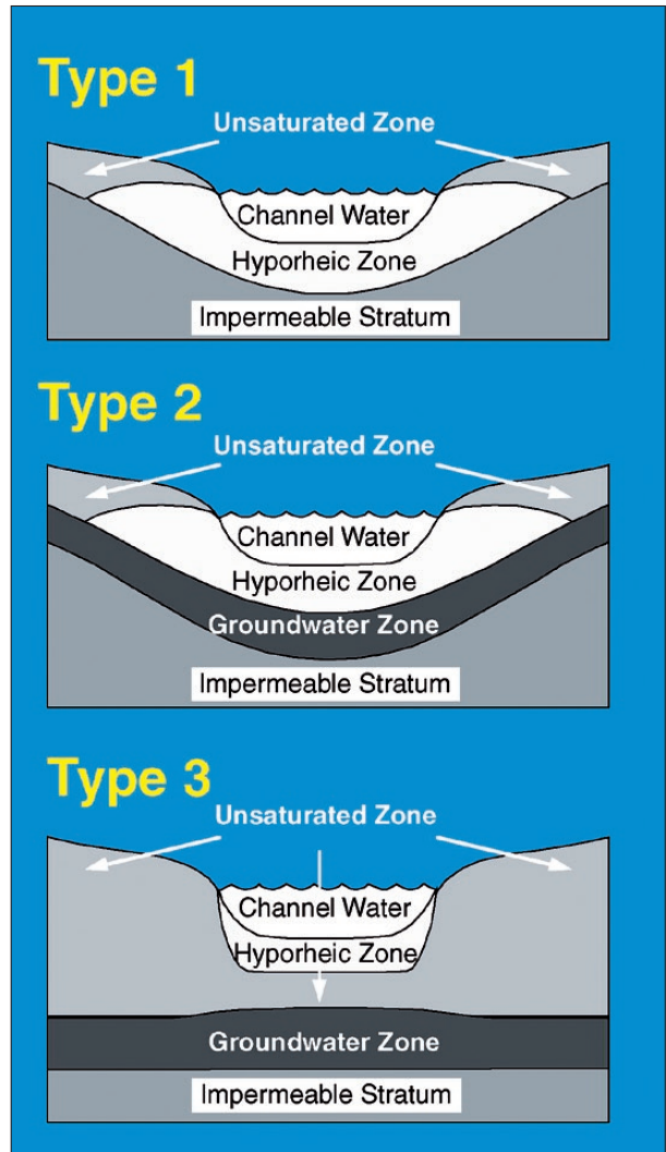
Fig. 4: Conceptual cross-sectional models of surface channels and beds showing the relationship of channel water to hypoheic, groundwater, and impermeable zones. From Malard et al. (2000).
