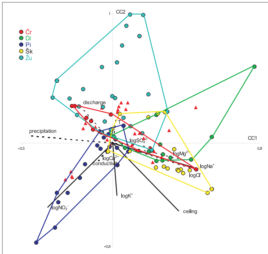
Fig. 8: Ordination diagram based on species composition and abundance data of copepods in epikarst drips showing caves (convex hulls containing sampling sites ○) and species (▲) in relation to the twelve environmental variables (represented as lines) of the five caves.
