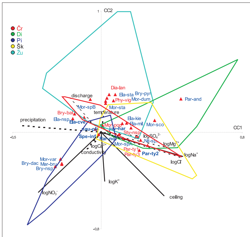
Fig. 9: Ordination diagram based on species composition and abundance data of copepods in epikarst drips in relation to the twelve environmental variables of the five caves. Species are abbreviated by the first three letters of the genus and species names. For complete names, see Pipan (2005) and Pipan et al. (2006).
