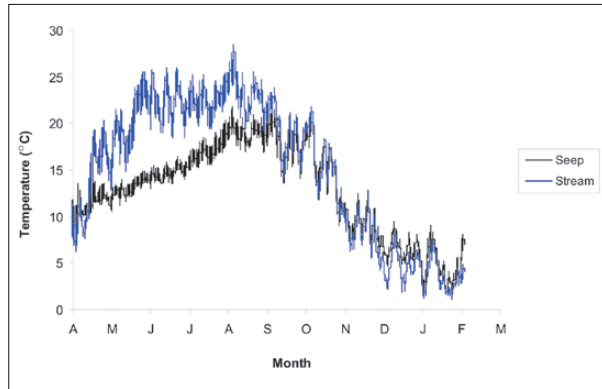
Fig. 6: Hourly temperatures from April 7, 2007 to February 4, 2008 in a seepage spring and adjoining stream in Prince William Forest Park, Virginia, USA. Because of the scale, the thickness of the line indicates the extent of daily fluctuations.
