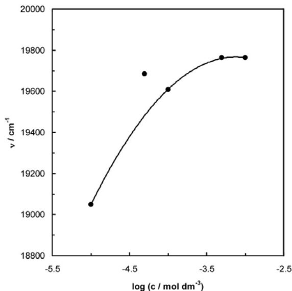
Figure 4: The effect of \beta -cyclodextrin on the position of the fluorescence maximum of coumarin 6 in water. \nu denotes the wave-number ( 1/\lambda ) of the fluorescence emission. The curve is provided to be a guide to the eye.
