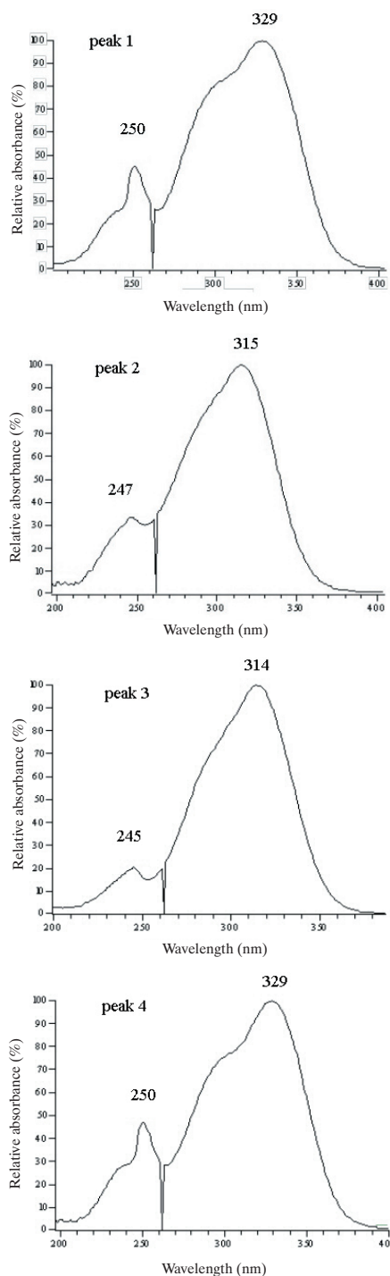
Figure 3. UV-Vis spectra of monitored HCAs in the Rebula grapes juice. The numbers correspond to the peaks of figure 2.
