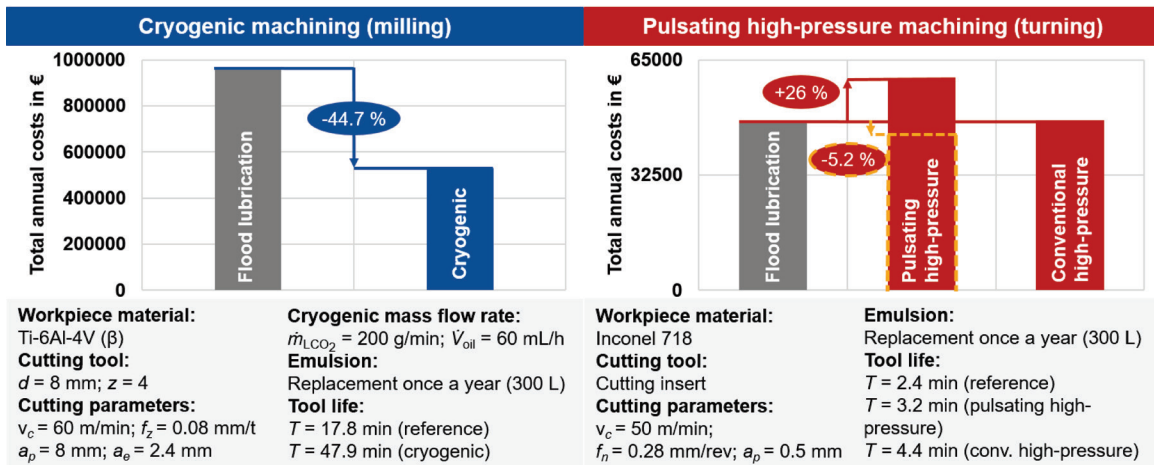
Fig. 9. Calculation of total annual costs for cryogenic machining and pulsating HPIAM
