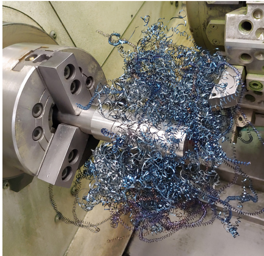
Fig. 10. Continuous chips wrapped around workpiece when turning AISI4142 alloy
