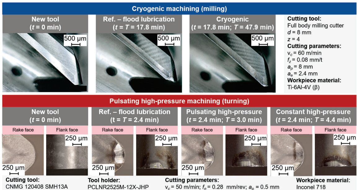
Fig. 5. Tool wear in cryogenic machining and pulsating HPIAM (t - time; T - tool life)
