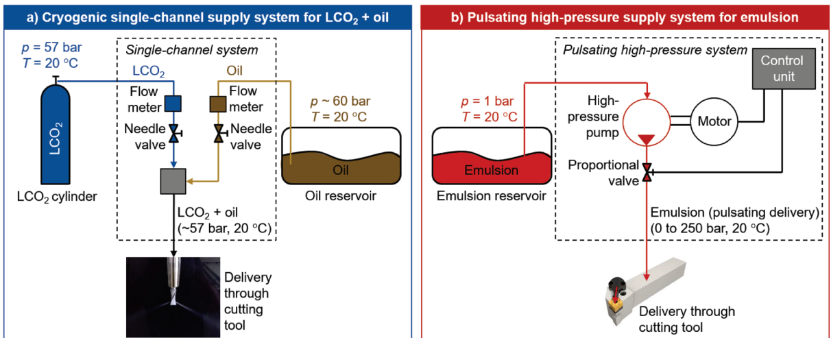
Fig. 4. Schematic setups a) for single-channel supply of LCO 2 +MQL; and b) pulsating HPIAM
