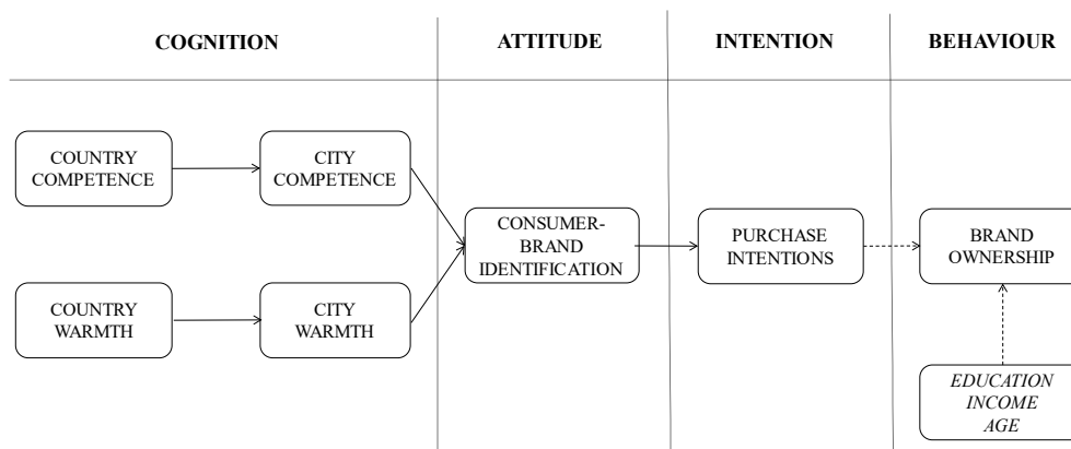
Figure 3: Conceptual model
