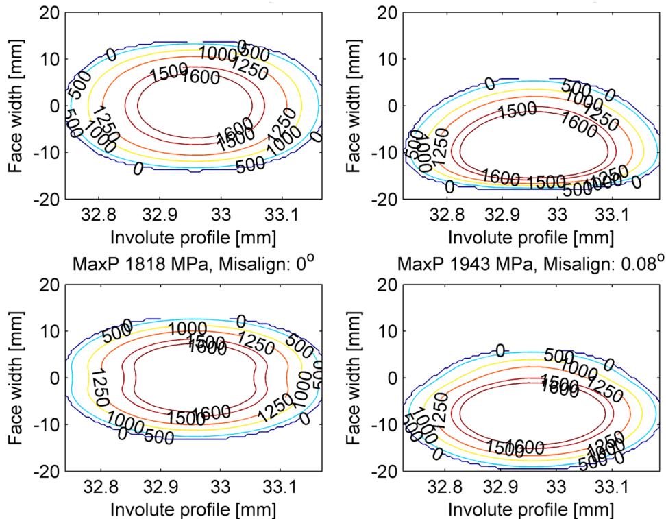
Fig. 5. Contact pressure distributions for the logarithmical profile (top) and parabolic modification (bottom) using an angular misalignment of 0^\circ and 0.08^\circ
