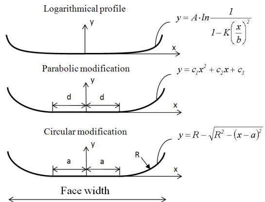
Fig.2 Schematic illustrations of all lead profiles. The x -axis represents the position at the face width and the y -axis the modified quantity
