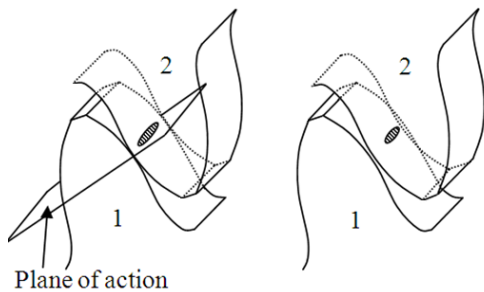
Fig. 1. Illustration of the gear contact with no misalignment (left) and with angular misalignment of gear 2 in the plane of action (right)
