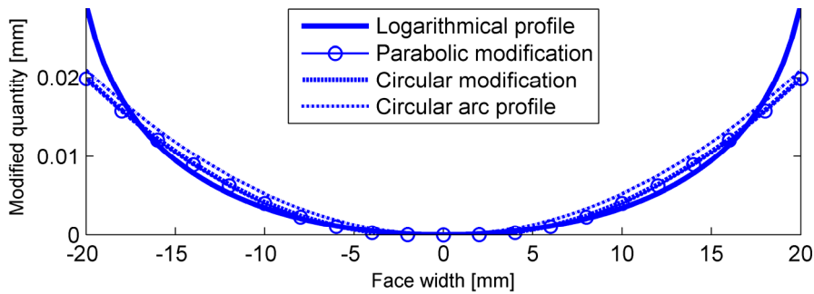
Fig. 3. Optimised lead profiles
