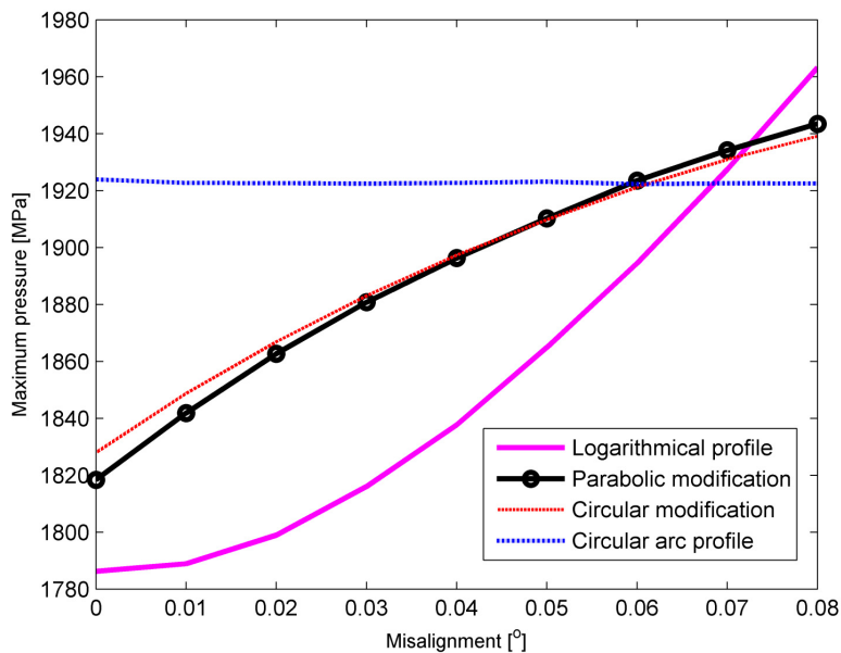
Fig. 4. The maximum contact pressure for all lead profiles versus the amount of misalignment
