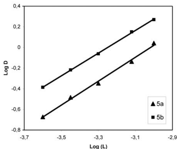
Fig. 1 \log D versus \log [L] for the extraction of Hg picrate by the ligands 5a and 5b from an aqueous phase into dichloromethane at 25 °C.
