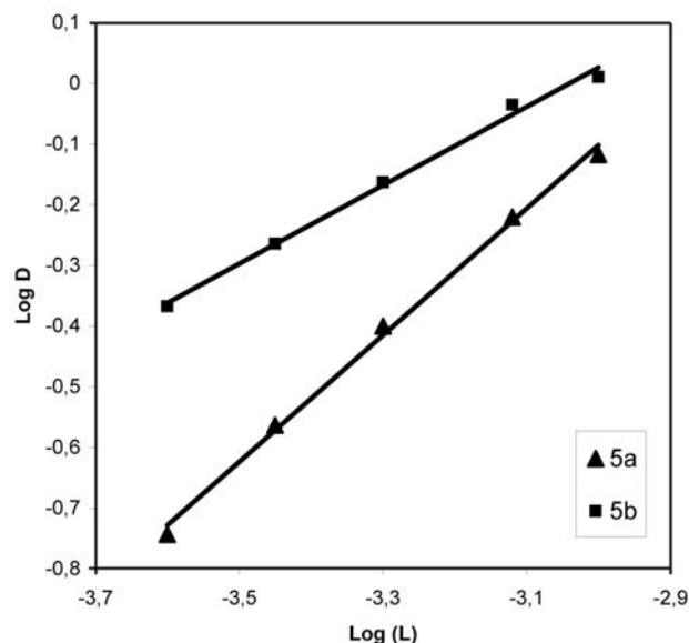
Fig. 3 \log D versus \log [L] for the extraction of dichromate anion by the ligands 5a and 5b from an aqueous phase into dichloromethane at 25 °C.
