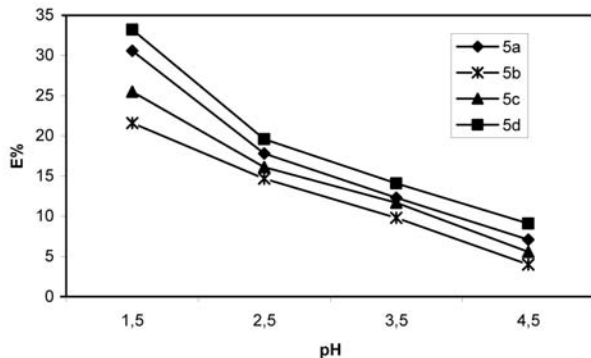
Fig. 2. Plots of extraction ( E %) versus pH following the two-phase solvent extraction of dichromate anion with compounds 5a-d .
