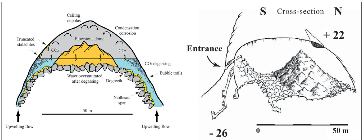
Fig. 40. The Champignons Cave, Provence, France, is an isolated chamber. Thermal hypogenic flow degassed CO 2 at shallow depth. Thermal convection enhanced condensation-corrosion to develop a large isolated chamber more than 50 m wide, which tends toward a hemispherical shape. Simultaneously, massive calcite deposits occurred in the lake, which was supersaturated with calcite because of CO 2 degassing (Audra et al. 2002).
