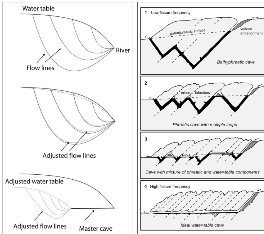
Fig. 2: Left: the water-table cave hypothesis proposed by Swinnerton (1932). Right: The four-state model of Ford and Ewers (1978). Depending on fissure frequency, various types of caves evolve: low fissure frequency (state 1) produces bathypneatic caves. With increasing fissure frequency the number of phreatic loops increases (states 2 and 3). High fissure frequency (state 4) results in water-table caves. Extremely low or extremely high fissure frequency does not allow evolution of caves (state 0 and 5, not shown here). The four states do not necessarily follow one another (after Ford 1999).
