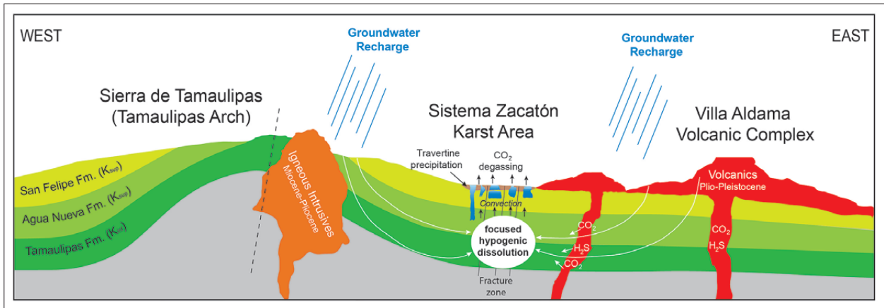
Fig. 32: Hypogenic speleogenesis of the Sistema Zacatón karst area. Groundwater flowpaths to Sistema Zacatón show enrichment of \text{CO}_2 and \text{H}_2\text{S} from the Pleistocene volcanic complex to the east. The main recharge area is located to the west in the Sierra de Tamaulipas. A fracture zone focused initial flowpaths. Heat source from volcanic activity drives convection in the groundwater system (Gary 2010). The combination of acids ( \text{H}_2\text{S} , \text{CO}_2 ), of thermalism, and of microbial activity is boosting dissolution along fractures acting as upflow paths. Giant ascending shafts are made by enlargement of fractures and by upward stoping of large chamber at depth that eventually open to the surface. This kind of “hyperkarst” generates the deepest phreatic shafts of the Planet.
