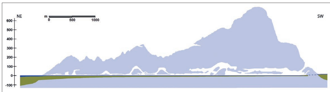
Fig. 13: Profile of Saint Paul Cave (Palawan Island, Philippines). The cave drains a polje at low altitude through a 6 km long passage along the water table and discharges to the sea (Piccini & Iandelli 2011).
