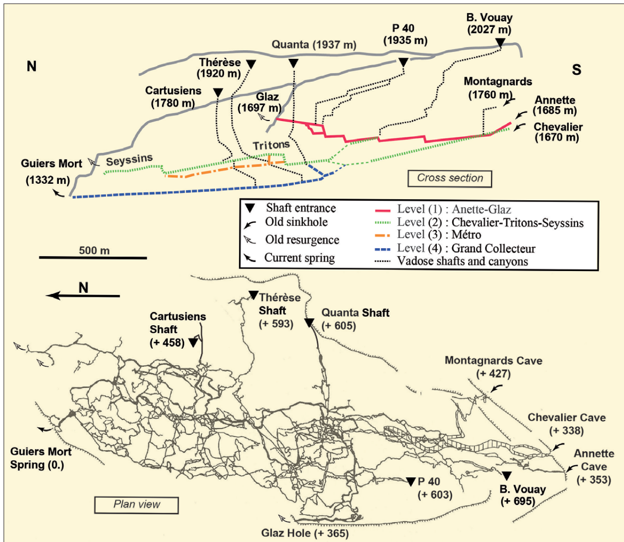
Fig. 14: The Dent de Crolles system, France, contains 57 km of passages over almost 700 m of depth, below a surface less than 1.5 km 2 in area. The cave consists of vadose shafts and canyons originating from the plateau surface, and which connect to four distinct semi-horizontally perched fossil galleries within the limestone mass; the lowest one, at the contact with the underlying aquiclude, is active.
