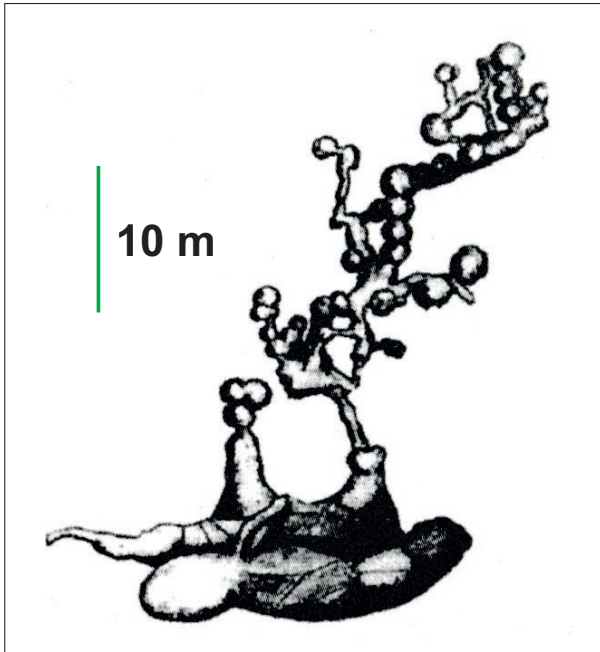
Fig. 39: Sátorkő-pusztá, Hungary. The “model” of hydrothermal cave, stacked spheres made by convective processes of sulfuric condensation-corrosion (Ford & Williams 2007).
