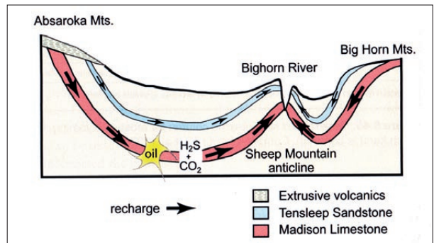
Fig. 26: The Bighorn River cut through the Sheep Mountain anticline allowing upflow of a deep aquifer discharging sulfuric water at Kane Caves, Wyoming, USA (Palmer & Palmer 2009, after Egemeir 1981).
