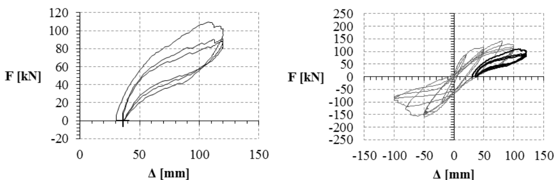
Slika 4.35: Histerezno obnašanje modela SIS-FRP v peti fazi Figure 4.35: Hysteretic behaviour of specimen SIS-FRP in fifth phase
