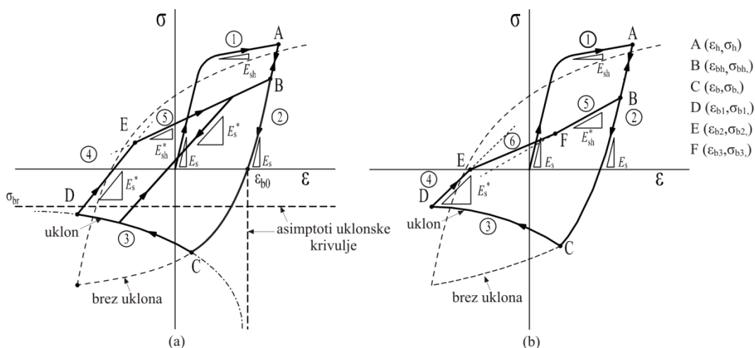
Slika 2.25: Histerezni model za zajem uklona za primer, ko \sigma_{bh} \geq \sigma_{b2} \geq 0 (a); in ko \sigma_{bh} \leq \sigma_{b2} ali \sigma_{b2} \leq 0 (b) (po Gomes in Appleton 1997; Tanoue et al. 2002)
