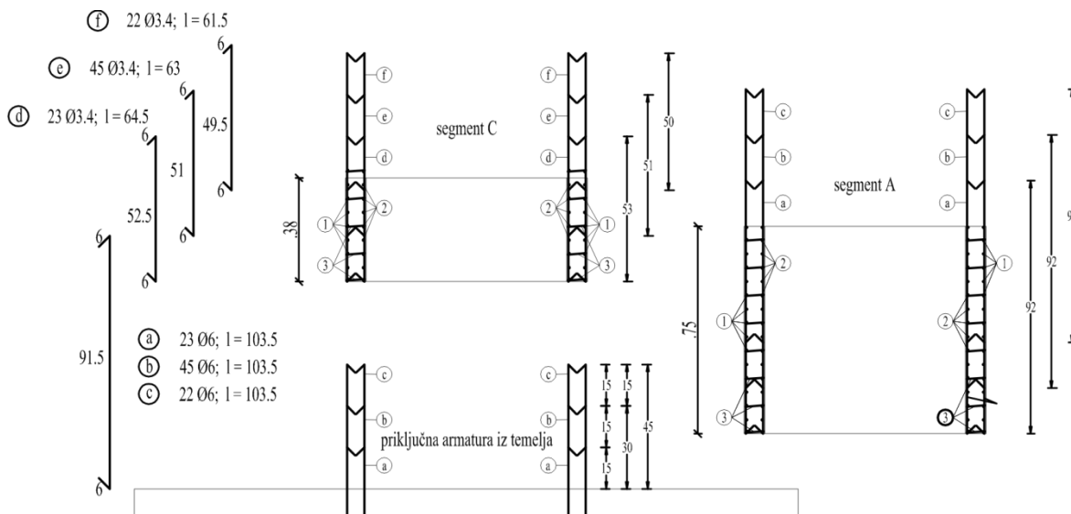
Slika 3.6: Armaturni načrt NKŠS; segmenta A in C Figure 3.6: Reinforcing plan for specimen NKŠS: segments A and C
