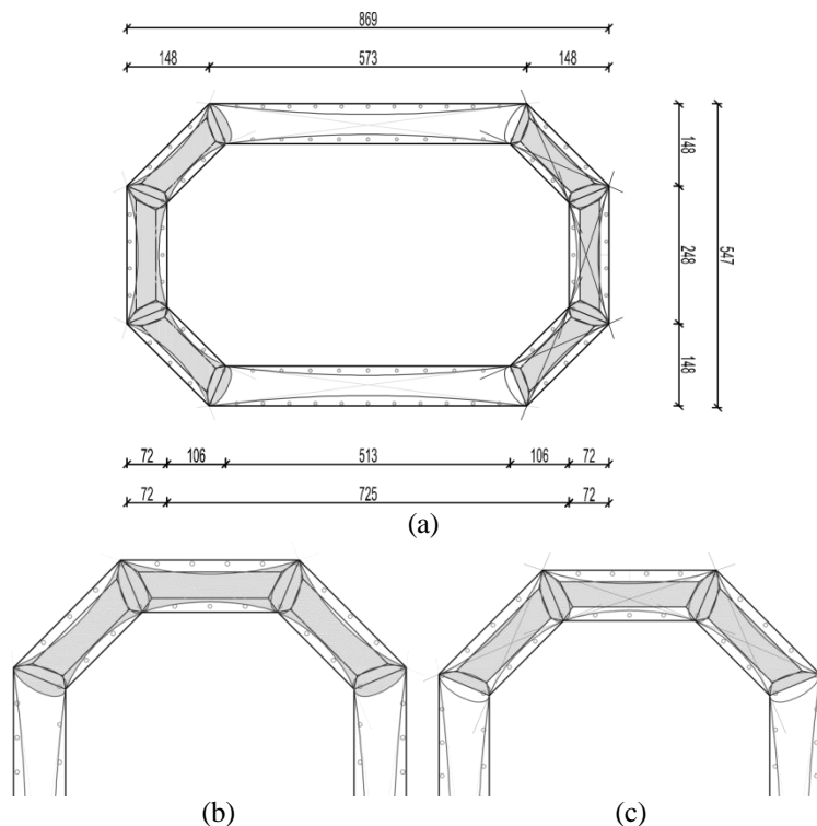
Slika 3.122: Modeliranje objetja v eksperimentalno preizkušenem stebru UKŠS-FRP (a); bližji pogled: ločni model (b); idealizacija za program OpenSees (c): šrafirano področje – objet beton Figure 3.122: Confinement modelling in experimentally tested specimen RK 4 (a); magnified view: arch model (b); idealization for OpenSees (c): hatched area – confined concrete
