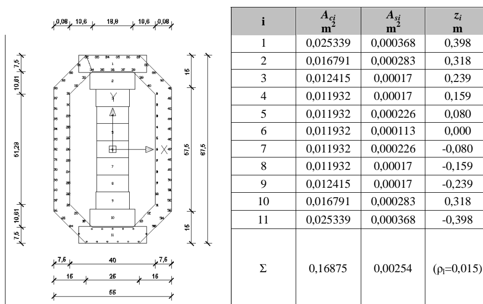
Slika 3.31: Delitev preseza na lamelle in njihove lastnosti za MVLEM element Figure 3.31: Section division to fibres and their properties for MVLEM element
