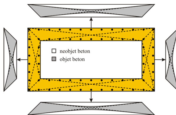
Slika 3.120: Škatlaste stebre obravnavamo kot sklop povezanih sten Figure 3.120: Hollow box columns are treated as set of connected walls
