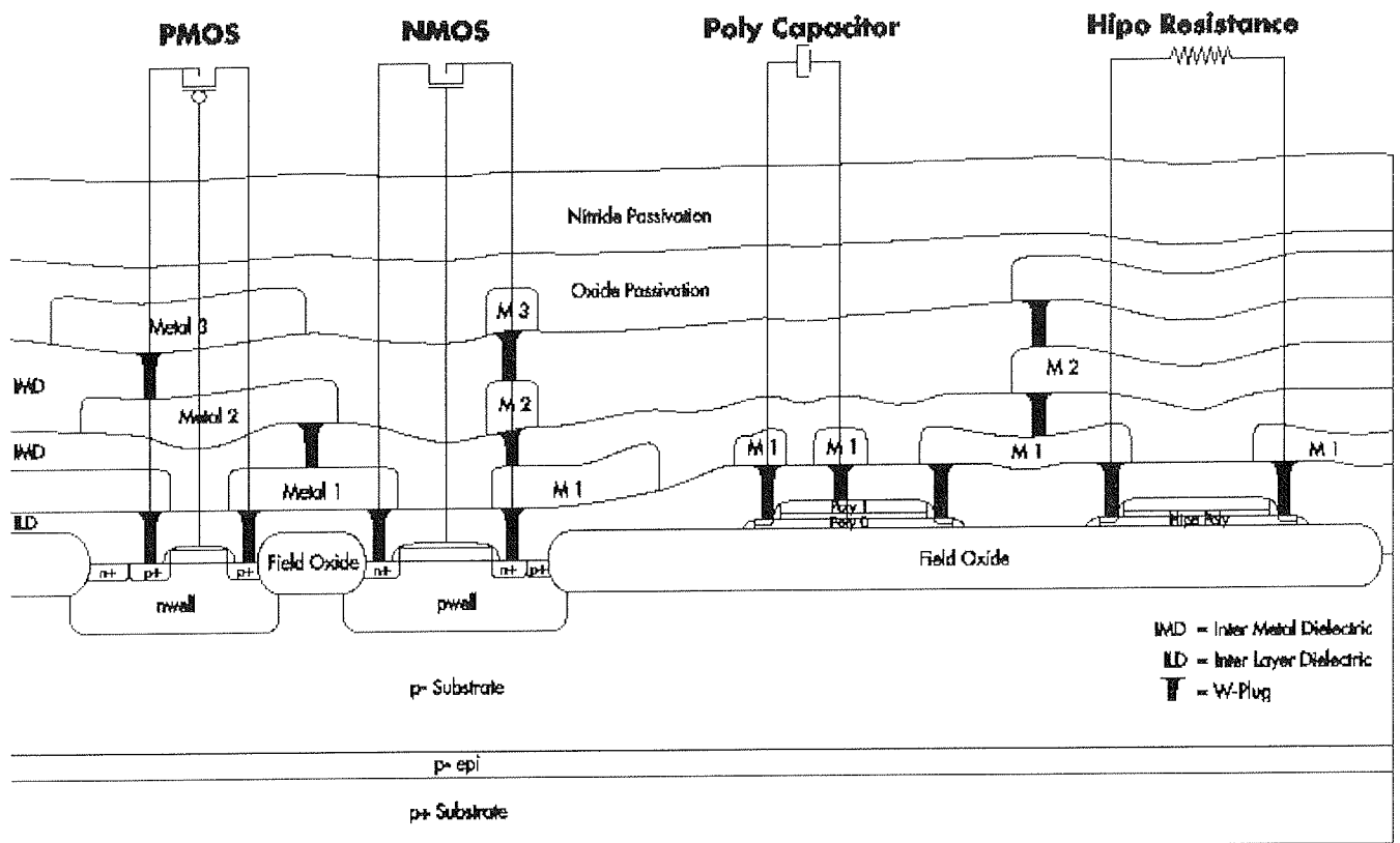
0.5 μ CMOS Cross Section
