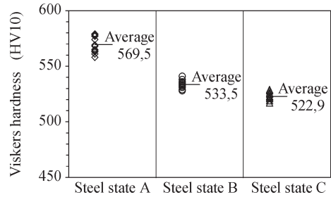
Fig. 9. Vickers hardness results of all three states
