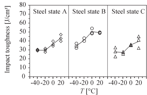
Fig. 10. Impact toughness of three states
