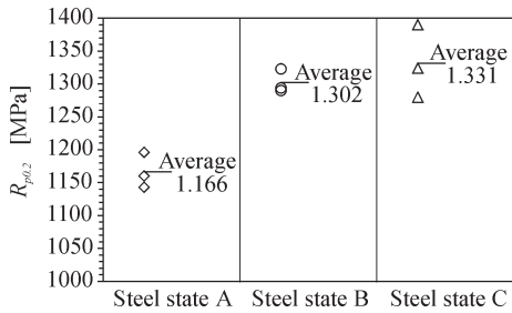
Fig. 5. Yield stress of three different states
