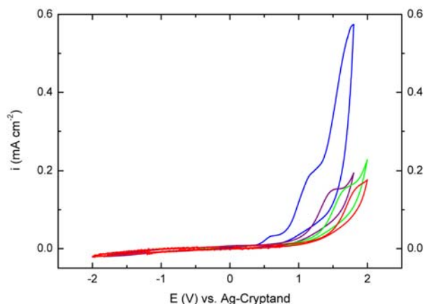
Figure 5: Cyclic voltammograms of a 1.2 M DMPBTFAc-AN solution on GC; ■ 1 st scan, ■ 2 nd scan, ■ 3 rd scan, ■ 4 th scan; scanning rate v = 5 \text{ mVs}^{-1}
