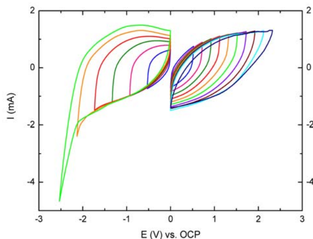
Figure 6: Cyclic voltammograms of a 1.0 M DMPBTFAc-AN solution on AC; scanning rate v = 5 \text{ mVs}^{-1}
