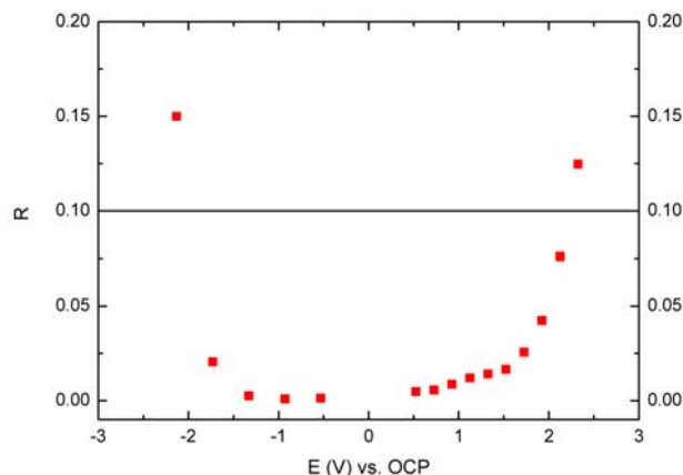
Figure 7: Faradaic Fraction R as a function of the potential for a 1 molal DMPBTFAc-AN solution on AC electrode; ■ Faradaic Fraction R , — limit according to Jow, for details see text.
