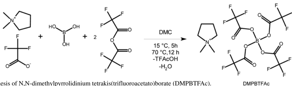
Figure 1: Synthesis of N,N-dimethylpyrrolidinium tetrakis(trifluoroacetato)borate (DMPBTFAc).
