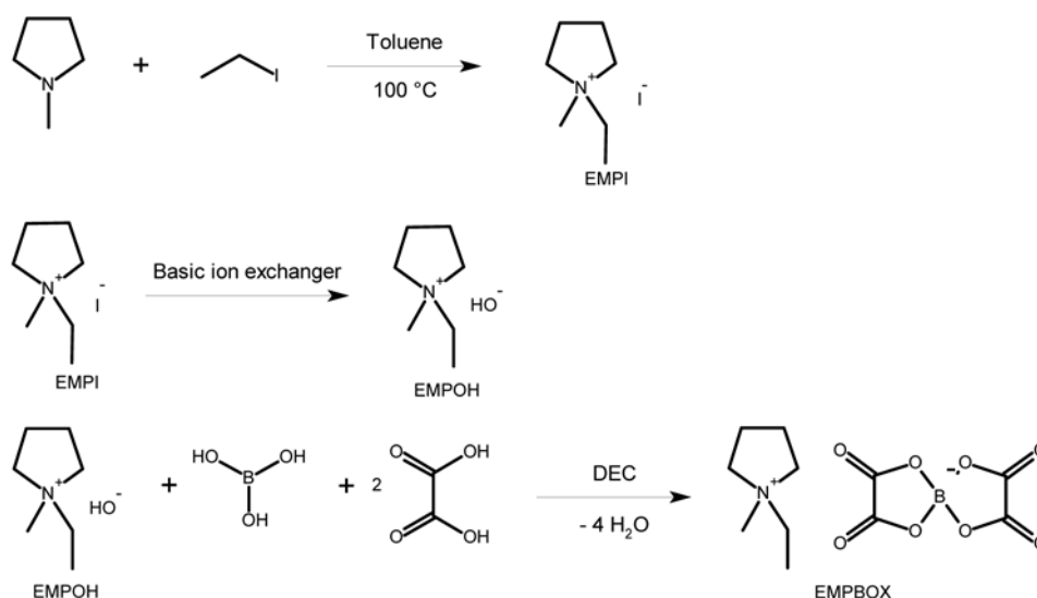
Figure 2: Synthesis of N-ethyl-N-methyl-pyrrolidinium bis[1,2-oxalato(2-O,O')]borate (EMPBOX).
