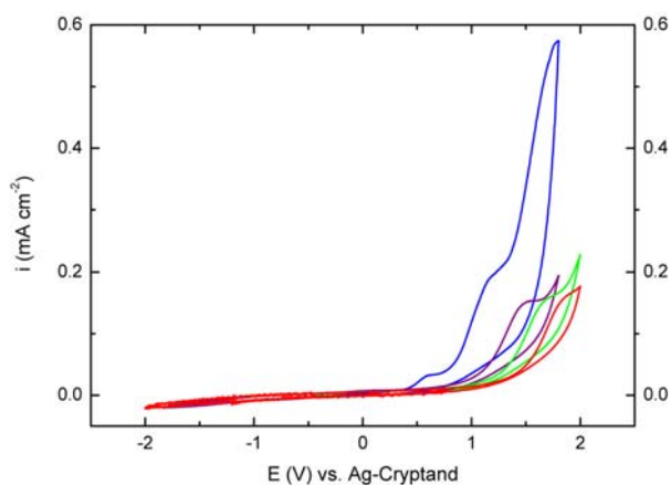
Figure 4: Cyclic voltammograms of a 1.2 M DMPBTFAc-AN solution on an Al-strip electrode ■ 1 st scan, ■ 2 nd scan, ■ 3 rd scan, ■ 4 th scan; scanning rate v = 5 \text{ mVs}^{-1}
