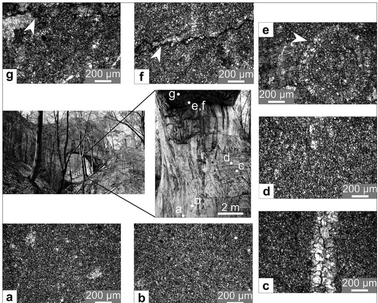
Fig. 5: Samar natural bridge from the NE Kučaj Mountains (Carpatho-Balkanides, eastern Serbia) and thin-section photomicrographs of the Late Jurassic limestones showing characteristic recrystallized fabrics of the Samar natural bridge. a) microsparite resulted by aggrading recrystallization of the former micritic matrix, sample SP 1. b) recrystallized cement with no preserved relics, sample SP 2. c, d) recrystallized cement with vein filling by sparry calcite fabric, c, sample SP 3; d, sample SP 4. e) recrystallized cement. The outline of the circle structure suggests a crinoids? whose skeleton has been replaced by calcite (white arrow), sample SP 5. f, g) low amplitude stylolites in a recrystallized cement (white arrows). The dark stylocumulate consists of Fe-oxides, f, sample SP 5; g) sample SP 6.
