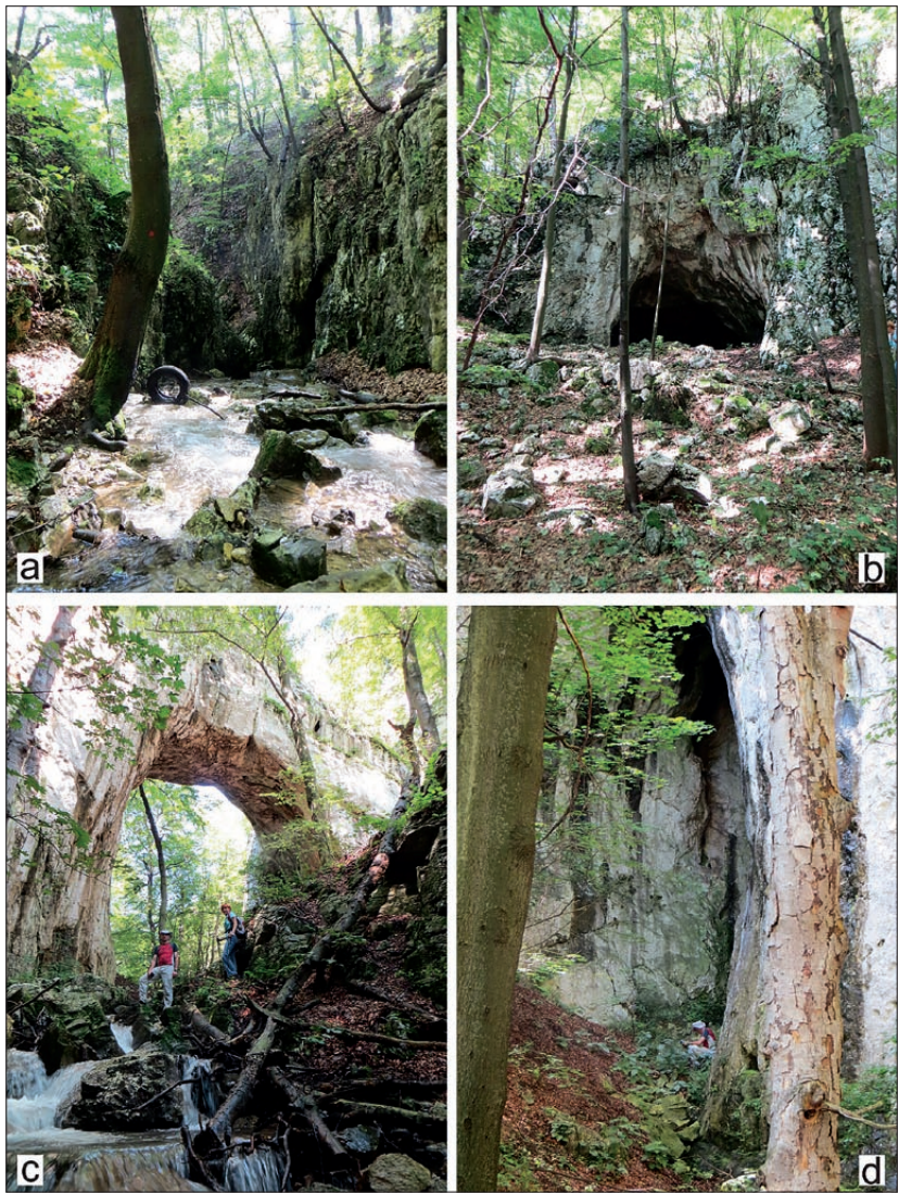
Fig. 4: Remains of a former cave in Ravna River valley. a, narrow part on entrance in gorge of Ravna River; b, entrance in side cave channel at the beginning of canyon; c, natural bridge Samar; d, entrance in cave situated in the right wall of Samar natural bridge (photographs by A. Petrović).
