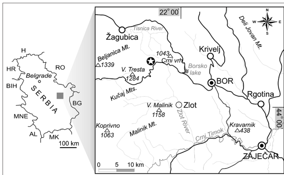
Fig. 1: Location map of the Ravna River doline and Samar natural bridge (star) from the NE Kučaj Mountains (Carpatho-Balkanides, eastern Serbia).
