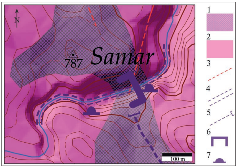
Fig. 3a: Geomorphological map of Ravna River collapse valley: 1, recrystallized carbonate rocks; 2, carbonate rocks; 3, fault, approximately located; 4, collapse valley (gorge); 5, hanging valley; 6, Samar natural bridge; 7, cave.
