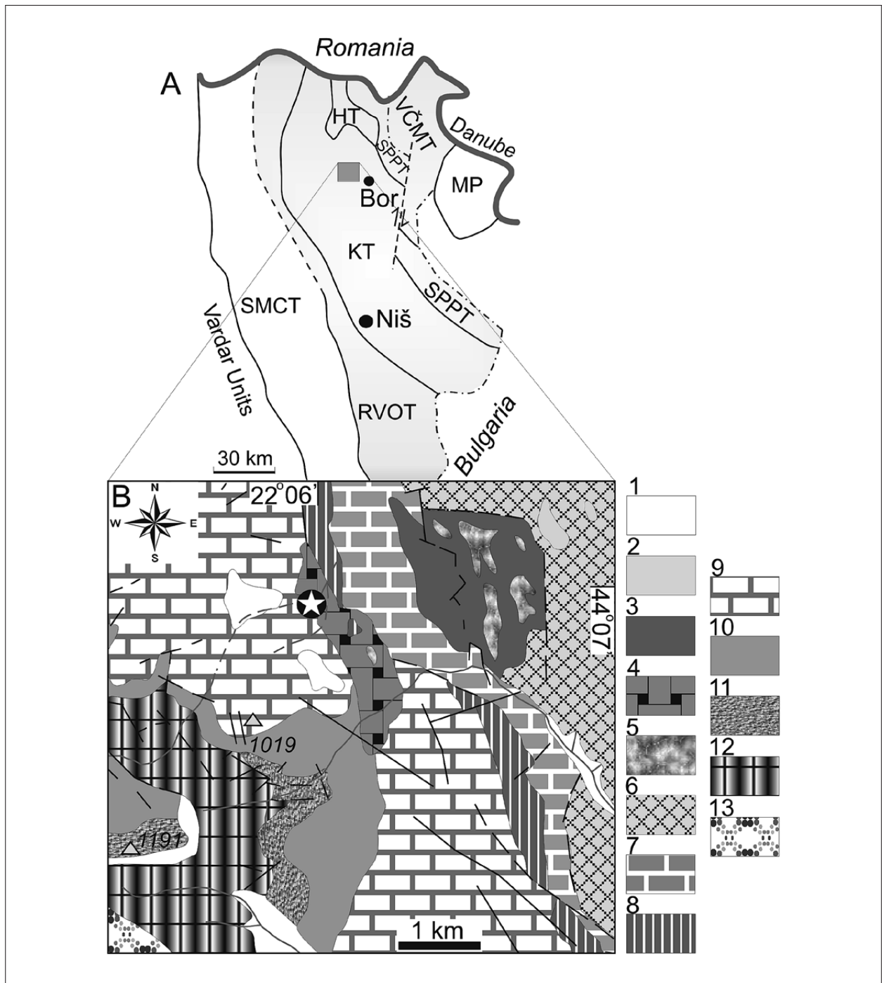
Fig. 2: a) Location map of the Ravna River valley and Samar natural bridge (star) from the NE Kučaj Mountains (Carpatho-Balkanides, eastern Serbia). b) Locality map of the investigated area in eastern Serbian Carpatho-Balkanides. A, Composite terranes of eastern Serbian Carpatho-Balkanides (shaded) as part of Balkan peninsula after Karamata & Krstić (1996): VČMT, Vrska Čuka-Miroč terrane; SPPT, Stara Planina-Poreč terrane; KT, Kučaj terrane; HT, Homolje terrane; RVOT, Ranovac-Vlasina-Osogovo terrane; MP, Moesian plate; SMCT, Serbian-Macedonian composite terrane. B, Geological map of the wider area of investigated locality (locality indicated by star) modified after Antonijević et al. 1970. 1, Quaternary deposits; 2, Paleogene dacitic-andesitic rocks; 3, Paleogene pyroclastics; 4, Paleogene skarns, marbles, hornfels; 5, Paleogene granites; 6, Upper Cretaceous volcanic agglomerate, breccia, tuffs, marly limestones; 7, Urgonian limestones; 8, "Neocomian" limestones; 9, Tithonian reef limestones; 10, Oxfordian and Kimmeridgian limestones with cherts; 11, Undifferentiated Middle and Upper Jurassic limestones; 12, Ordovician metasandstones and argillites; 13, Precambrian schists.
