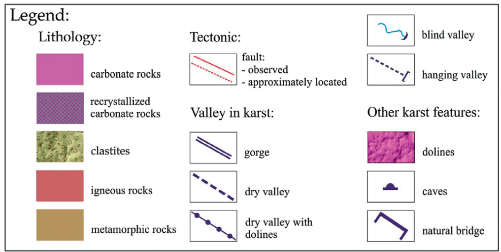
Fig. 3: Geomorphological map of Ravna River drainage area (yellow line) and its surrounding.
