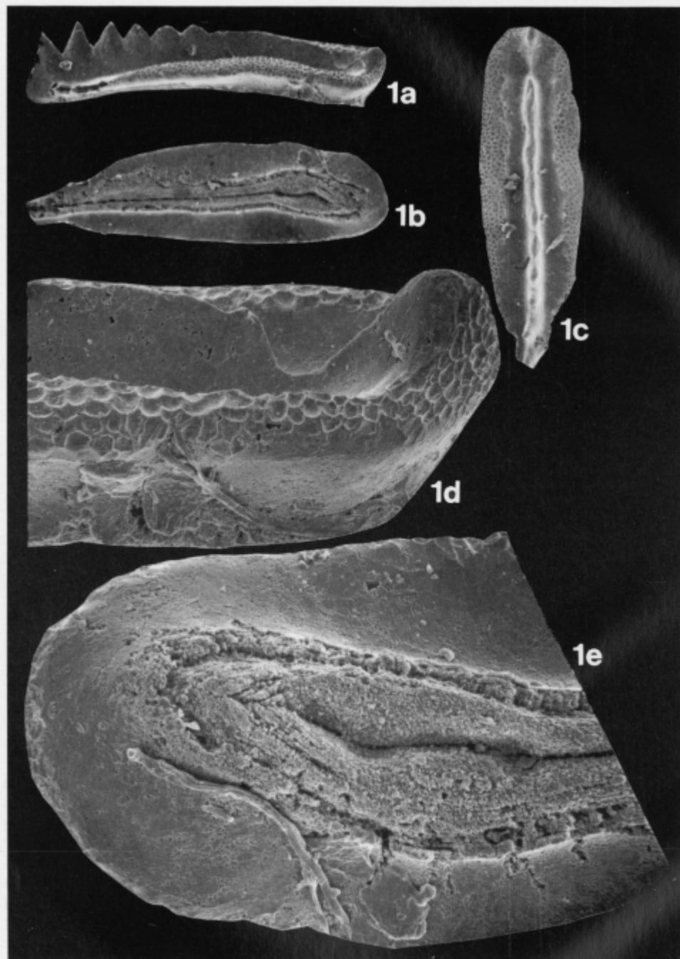
time the Rastdorf Group (Lower Pseudoschwagerina Limestone, Gersdorf Formation)
