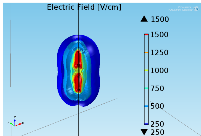
Figure 2: Electric Field distribution resulting from a bipolar electrode with an applied voltage of 1250 V.
