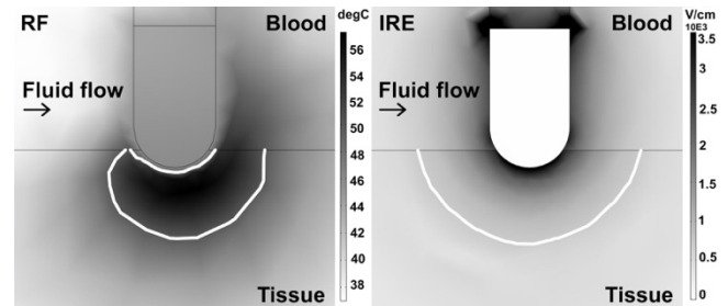
Figure 1: (RF) Temperature solution of radiofrequency model. White line shows the boundary at 50 ^{\circ} C. (IRE) Electric field solution of irreversible electroporation model. White line shows the boundary at 700 V/cm.
