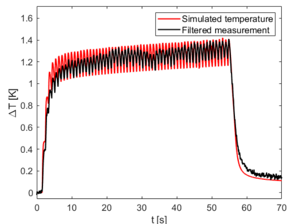
Figure 1: Comparison of simulated and measured temperature change within the outlet channel of large parallel plate treatment chamber. Pulse protocol: U_m = 1000 V, \tau = 100 \mu\text{s} , f = 1.1 Hz, F = 20 ml/min.
