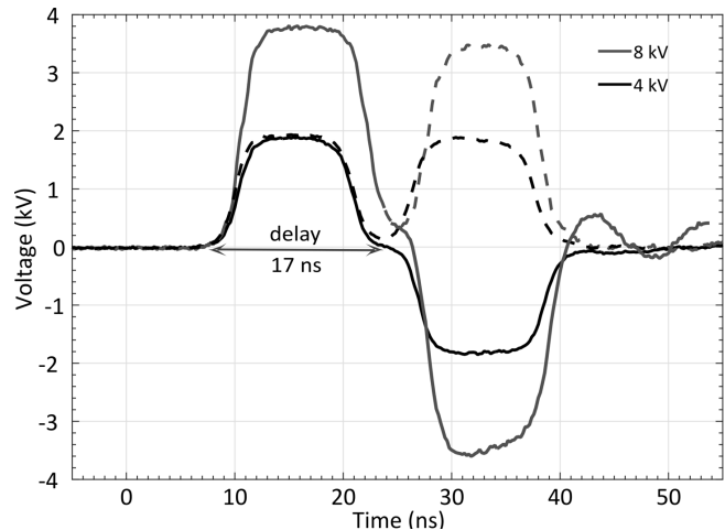
Figure 1: 10-ns bipolar (solid lines) and paired (dashed lines) pulses with a delay of 17 ns. Bias voltage is set to 4 (black lines) and 8 kV (gray lines).
