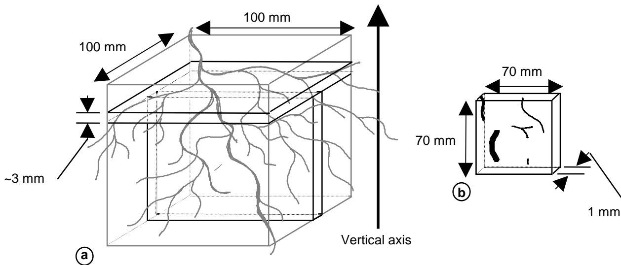
Figure 1. Schematic representation of the sectioning method to obtain vertical and horizontal sections from an impregnated soil sample (a), and actual dimensions of the sections used for subsequent imaging and analysis, (b)(the black fibres represent the sampled fraction of the initial root system).
