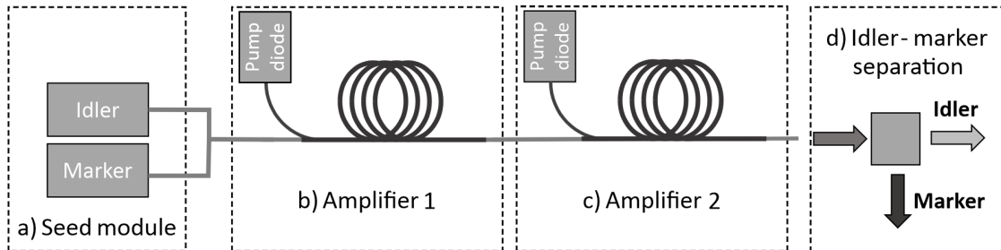
Fig. 3. The advanced system for pulse-on-demand generation; seed module a) consisting of the seed and marker laser diodes keeps the gain balance through the amplifiers b) and c) constant regardless of the marker pulse shape and repetition on the output; the marker and idler signals are separated at the output d) by the volume Bragg grating (VBG)
