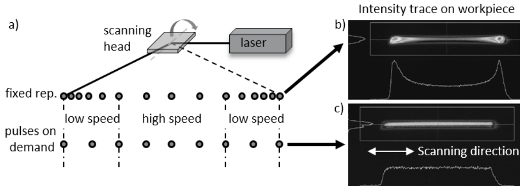
Fig. 6. a) Using a resonant scanner to generate a pattern with laser source operating at a fixed repetition rate captured on the beam profiler camera b); and with the laser source compensating the pulse delay to evenly distribute the laser power over the line trace c)
