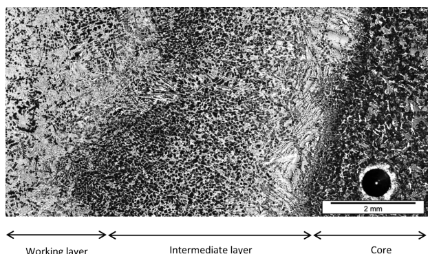
Figure 2: Macrostructure of the working layer, the intermediate layer and the core
