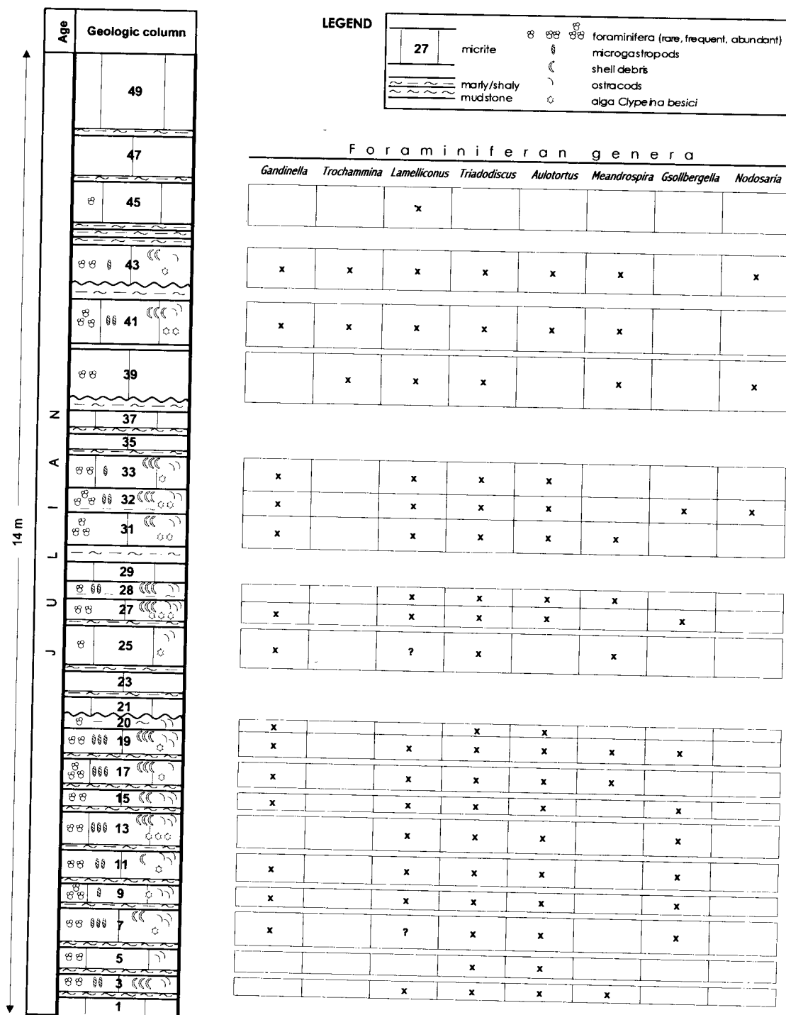
Fig. 2. Distribution of Foraminifera and other microfossils in the Kucler quarry section (The stratimetric column is modified after Jelen, 1990, p.24; strata are numbered on the field already)
