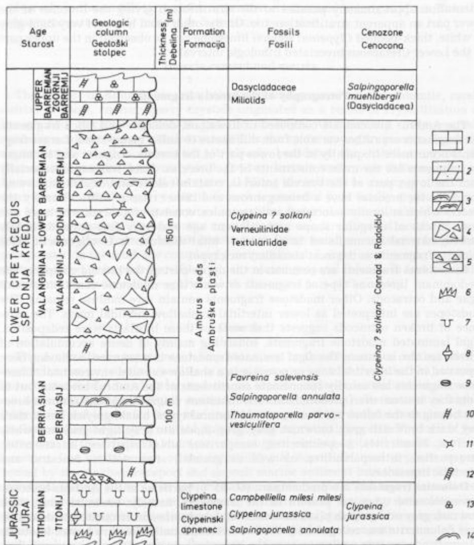
Fig. 2. Geologic column of the Ambrus beds in the Suha Krajina area
