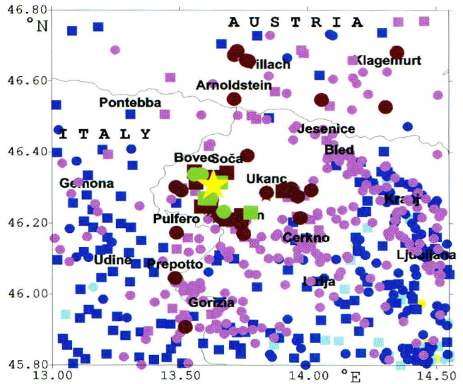
Figure 1a. Intensities of the earthquake on 12 April 1998 at 10:55 UTC.
