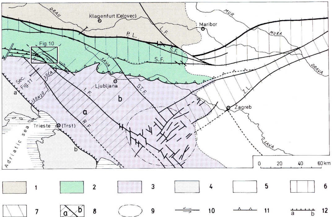
Figure 9: Neotectonic map of Slovenia and adjacent regions (after Placer 1999a,b). 1. Eastern Alps (Austroalpine); 2. Southern Alps; 3. External and Internal Dinarides; 4. Adriatic - Apulian foreland; 5. Pannonian basin; 6. Periadriatic tectonic zone; 7. Mid-Hungarian tectonic zone; 8. Idrija tectonic zone, a - outer part, b - inner part; 9. Idrija - Mid-Hungarian Transection zone; 10. recent active strike-slip fault; 11. Southalpine thrust front; 12. External Dinaric thrust front (a - Palmanova line, b - Karst thrust brink); P.L. Periadriatic lineament; S.F. Sava fault; Š.F. Soštanj fault; L.F. Lavant fault; Z.L. Zagreb lineament; ST.F. Stična fault; I.F. Idrija fault; R.F. Raša fault.
