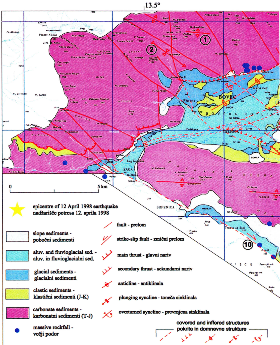
Figure 10: Generalised geological map of Upper Soča Valley (after Kuščer et al., 1974, Buser, 1987, Jurkovišek, 1987a, Poljak et al., 1998). Numbers in open circles: 1. Rombon anticline, 2. Kanin syncline, 3. Mojstrovka fault, 4. Soča fault, 5. Vrata fault, 6. Krm overthrust, 7. Polovnik anticline, 8. Kneža fault, 9. Ravne fault, 10. Idrija fault, 11. Bovec syncline
