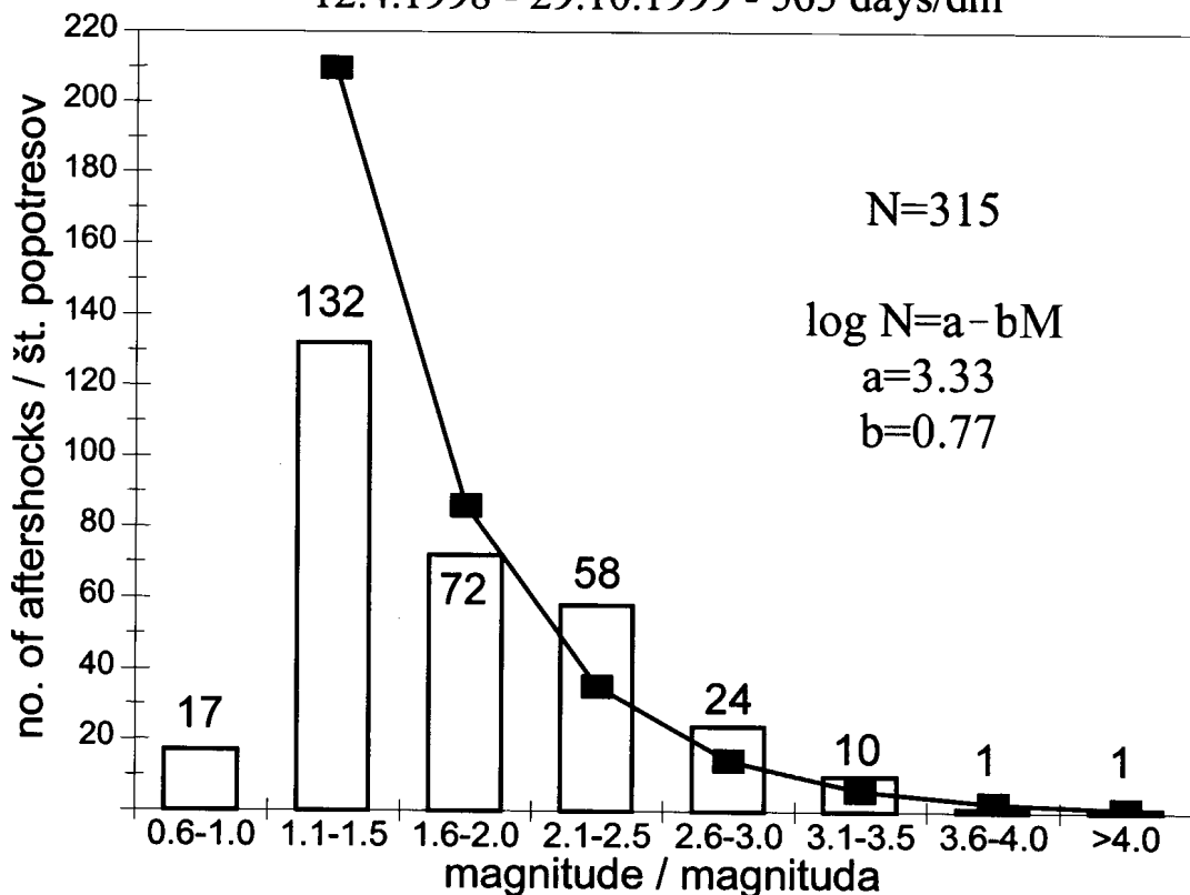
Figure 3. Magnitude-frequency relation (bar) for aftershocks with fitted Gutenberg-Richter's function (line).
