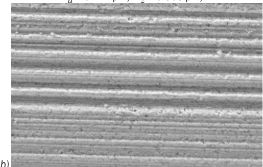
b) a_p = 0.01 \text{ mm} , f = 0.005 \text{ mm/rev} , v = 40 \text{ m/s} , R_a = 0.063 \text{ }\mu\text{m} , R_z = 0.290 \text{ }\mu\text{m} ;
