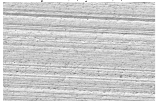
c) a_p = 0.01 \text{ mm} , f = 0.005 \text{ mm/rev} , v = 55 \text{ m/s} , R_a = 0.057 \text{ }\mu\text{m} , R_z = 0.228 \text{ }\mu\text{m}
