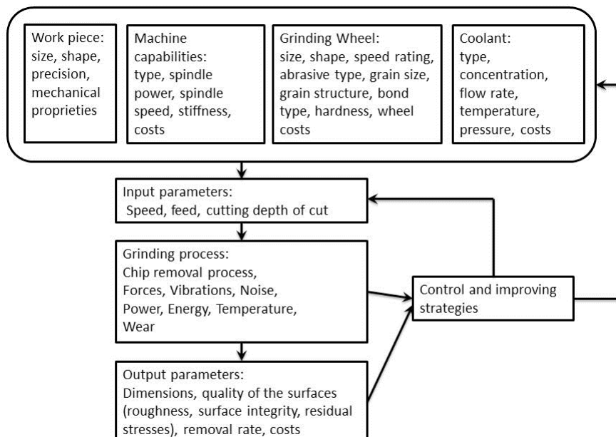
Fig. 2. Grinding model
