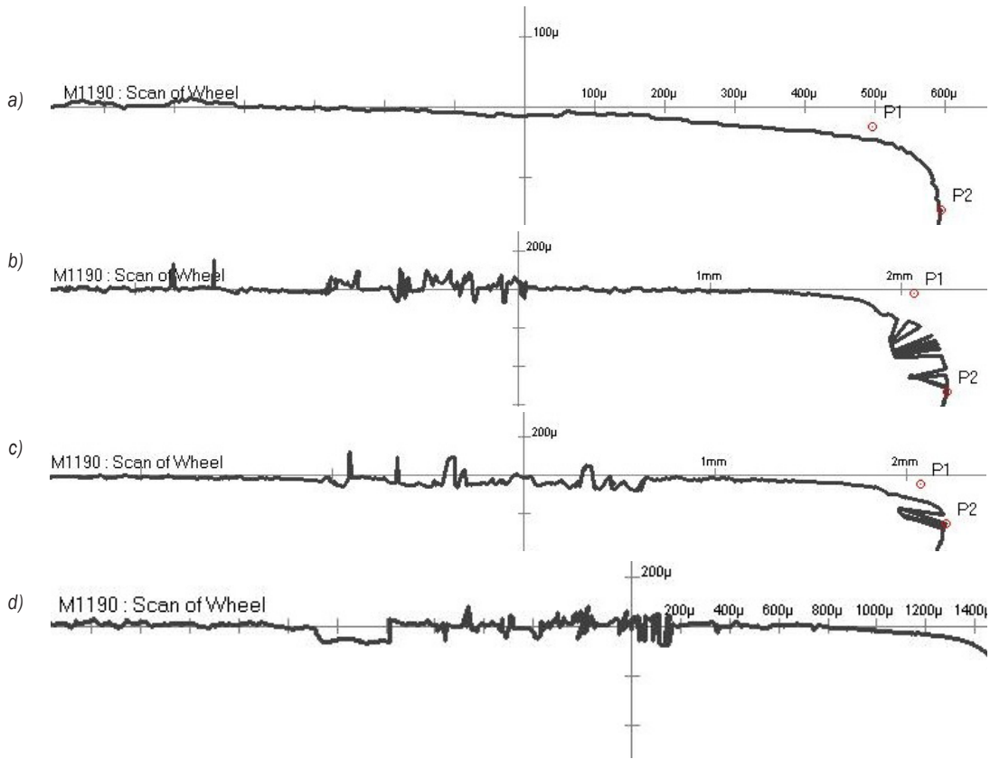
Fig. 6. Grinding wheel profiles with 54 \mu\text{m} grit a) unused wheel; b); c) and d) grinding wheel after sharpening of 300, 600, 800 gun drills
