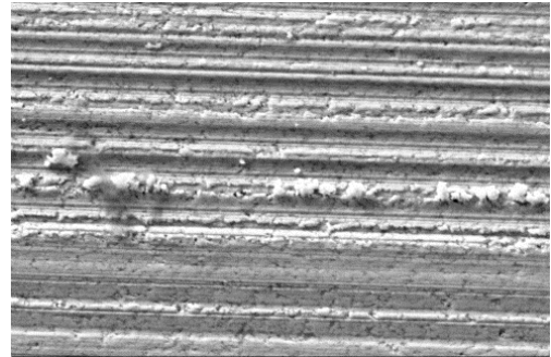
a) a_p = 0.03 \text{ mm} , f = 0.008 \text{ mm/rev} , v = 40 \text{ m/s} , R_a = 0.142 \text{ }\mu\text{m} , R_z = 0.568 \text{ }\mu\text{m} ,
