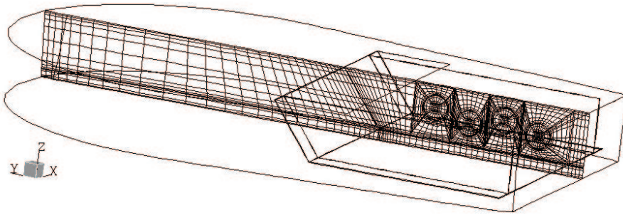
Figure 2: Computational mesh
