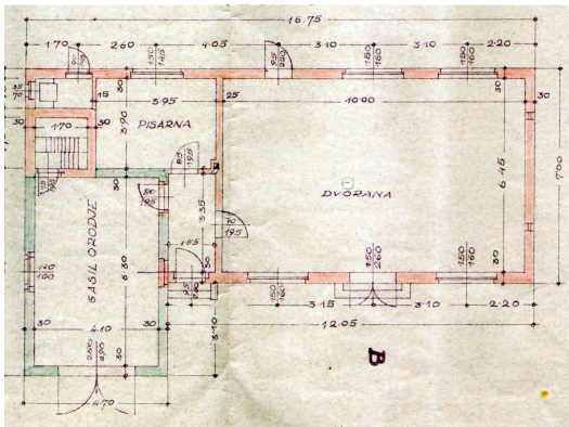
Tloris prizidka dvorane in stolpa
