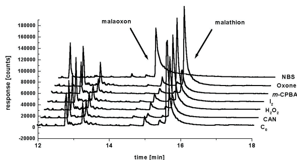
Figure 4. GC-MS chromatograms of malathion oxidation to malaoxon by various oxidants
