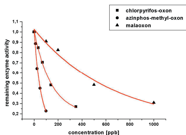
Figure 8. Inhibition curves for detection of malathion, chlorpyrifos and azinphos-methyl after oxidation to their respective oxons by the FIA AChE-TLS bioassay
