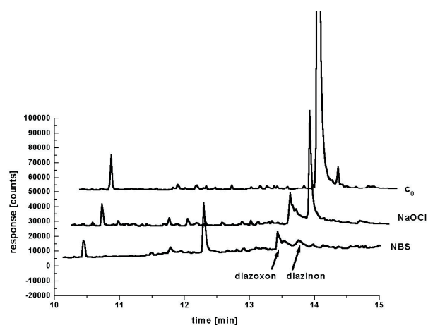
Figure 5. GC-MS chromatograms of diazinon oxidation to diazooxon by NBS and sodium hypochlorite
