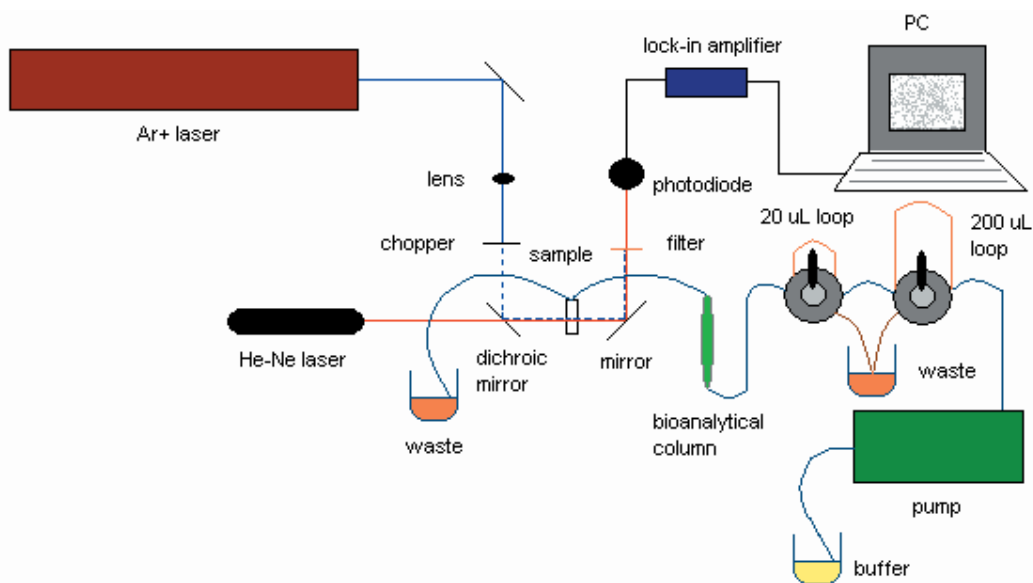
Figure 2. A schematic diagram of the bioanalytical FIA set up with TLS as a detection unit.
