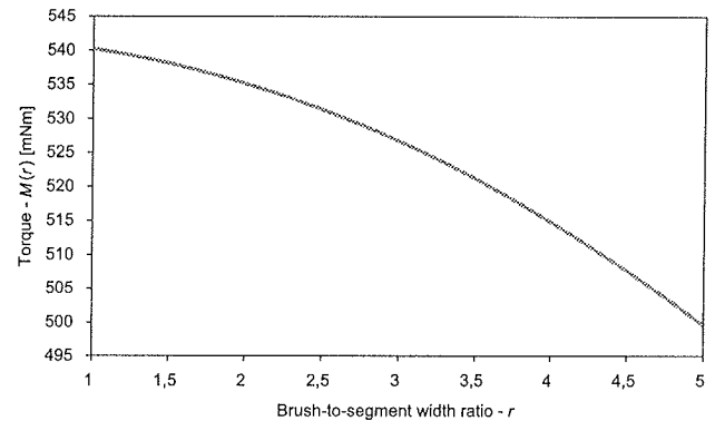
Fig.6: The torque M(r) , depending on the brush-to-segment width ratio, at the linear commutation.
