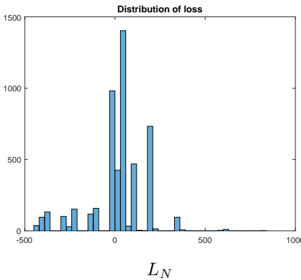
Figure 1: The distribution of final loss and optimal time \nu .
