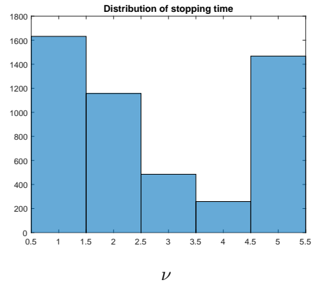
Figure 1: The distribution of final loss and optimal time \nu .
