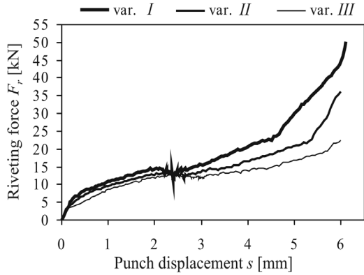
Fig. 8. A comparison of riveting force curve for three profiles (rivet mat. 1, \mu = 0.05 , \delta_t = 0.5 )
