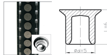
Fig. 3. Used rivet; a) real appearance, b) major dimensions
