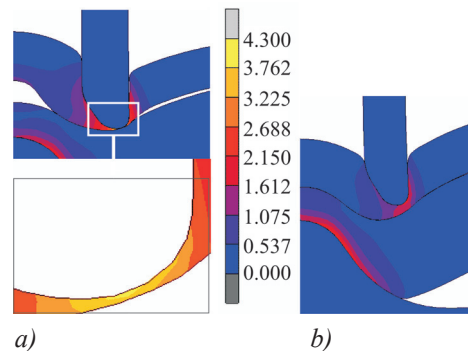
Fig. 14. The comparison of the equivalent plastic strain distribution and joint element deformation at the same punch path for the model with \mu between rivet and sheets; a) 0.05, b) 0.25 (die var. I, rivet mat. 4, \delta_t = 0.5 )
